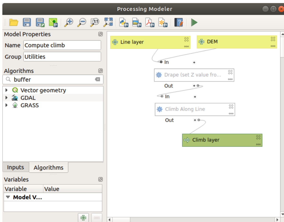
Рис. 21.23: A complete model
