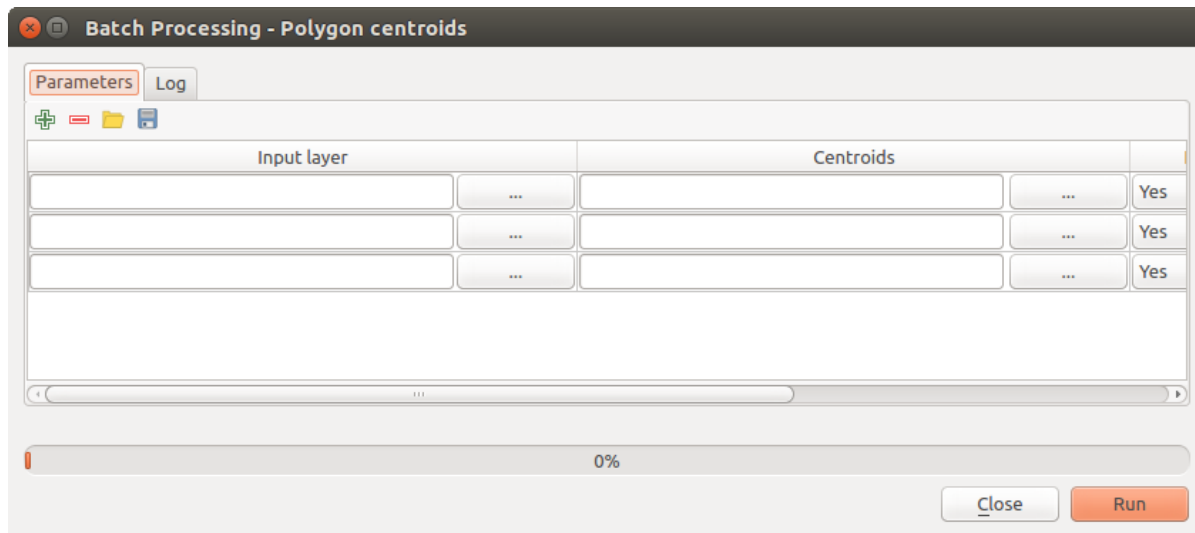
Рис. 21.30: Batch Processing
