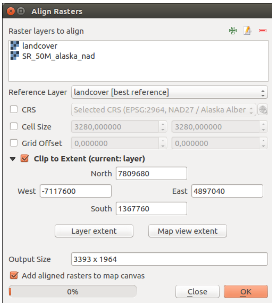
Рис. 14.16: Raster Alignment
