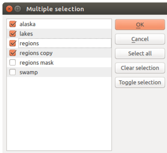
Рис. 21.14: Multiple Selection
