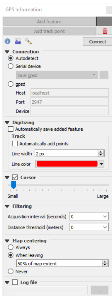
Рис. 18.5: GPS tracking options window
