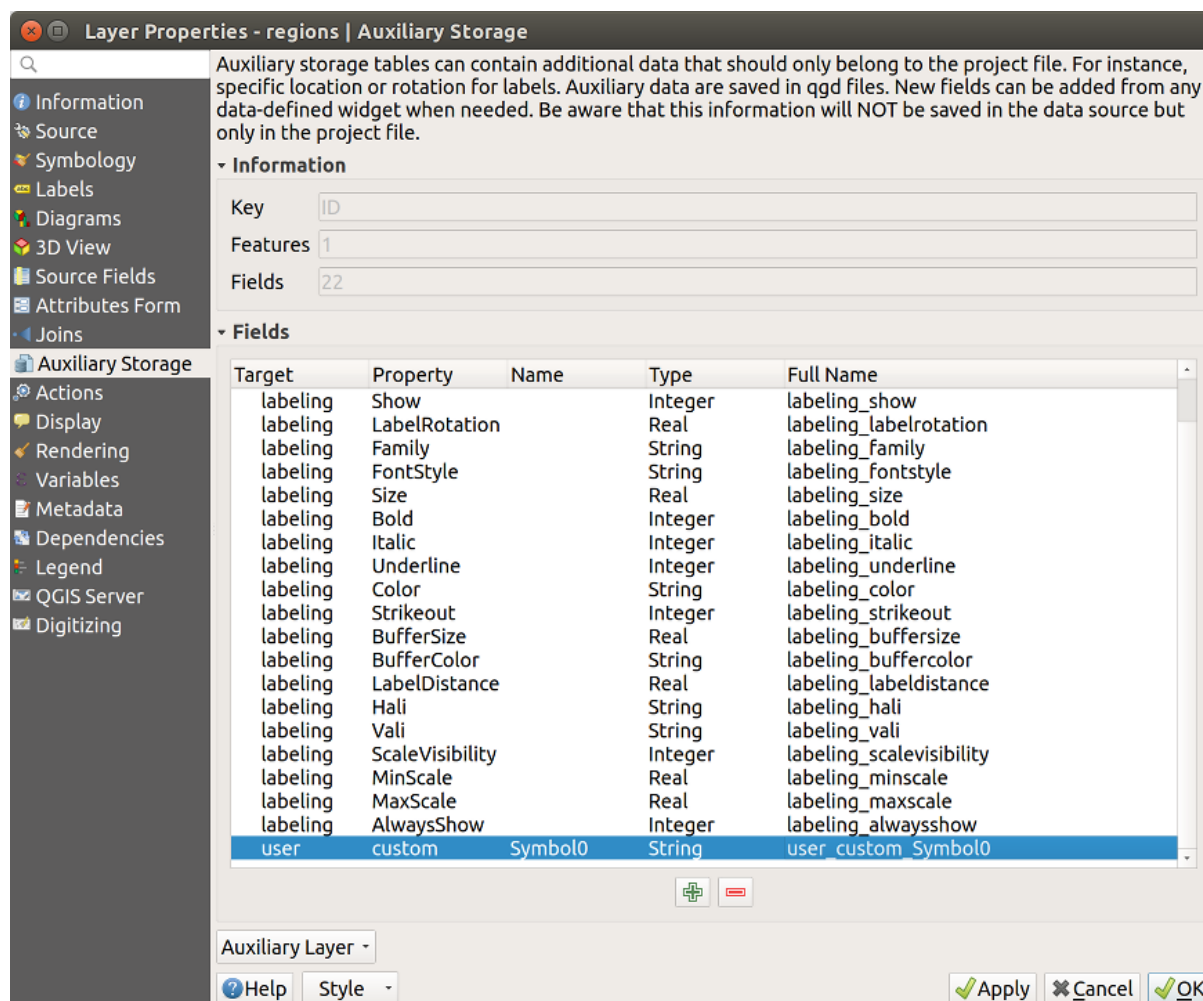
Рис. 13.61: Auxiliary field symbol
