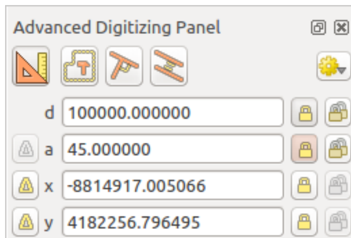
Рис. 13.101: The Advanced Digitizing panel
