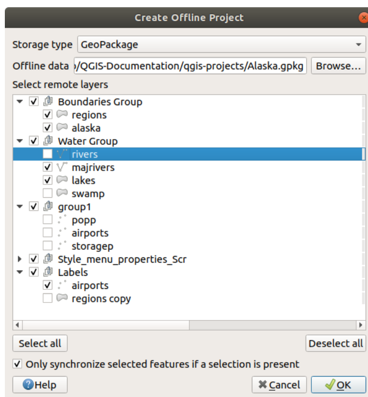
Рис. 22.27: Create an offline project
