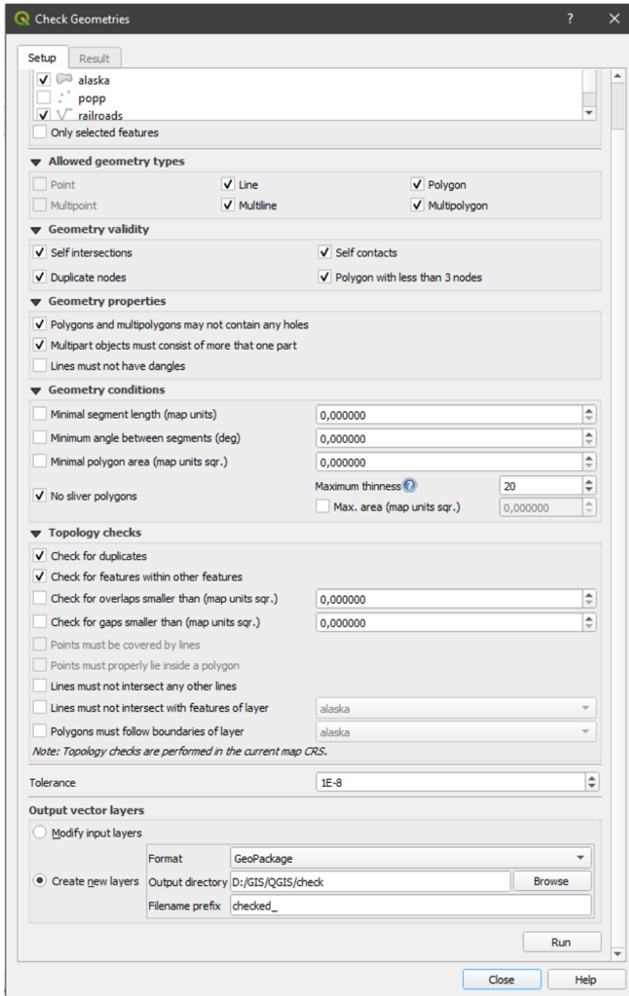
Рис. 22.17: The Geometry Checker Plugin
