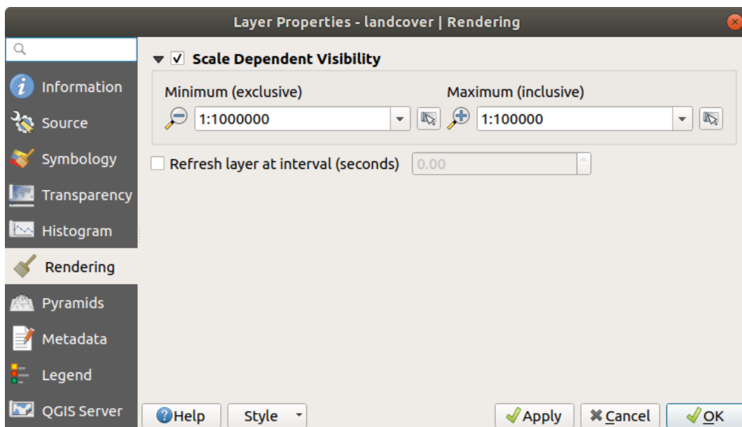
Рис. 14.11: Raster Rendering
