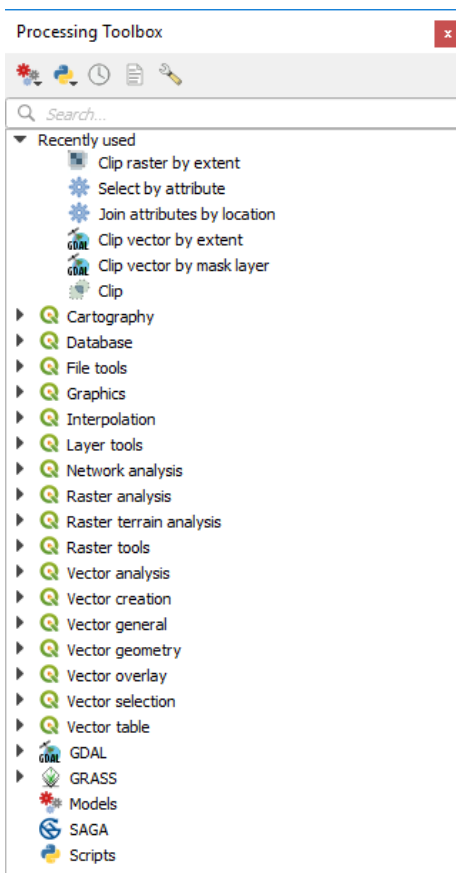
Рис. 21.6: Processing Toolbox
