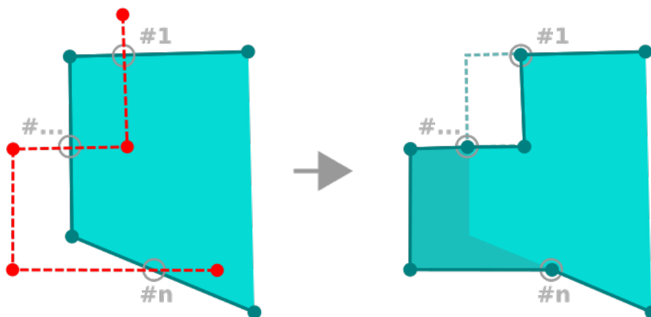
Рис. 13.99: Reshape polygon
