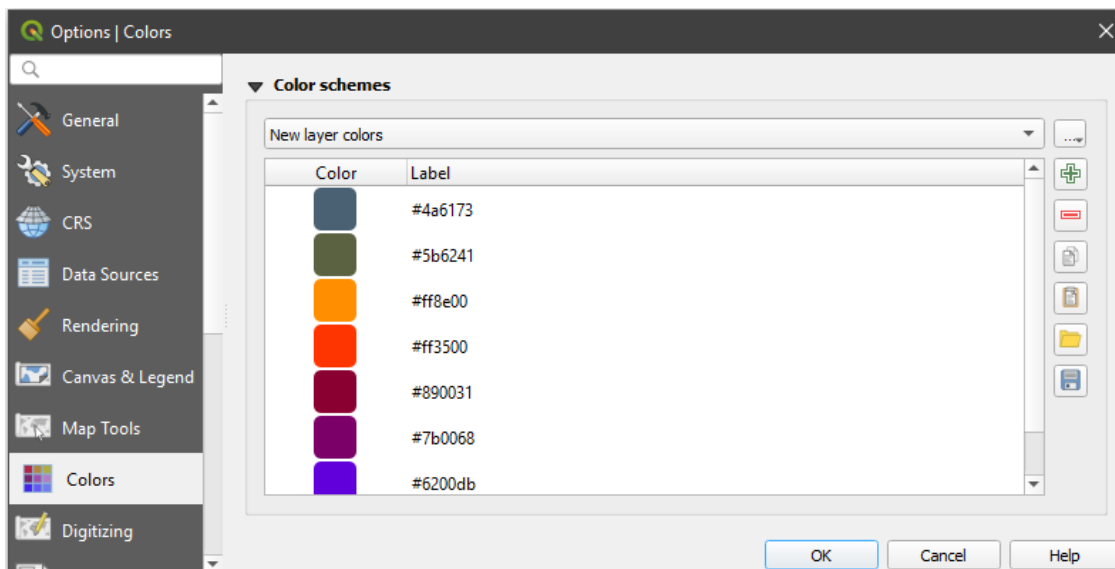
Рис. 9.7: Colors Settings
