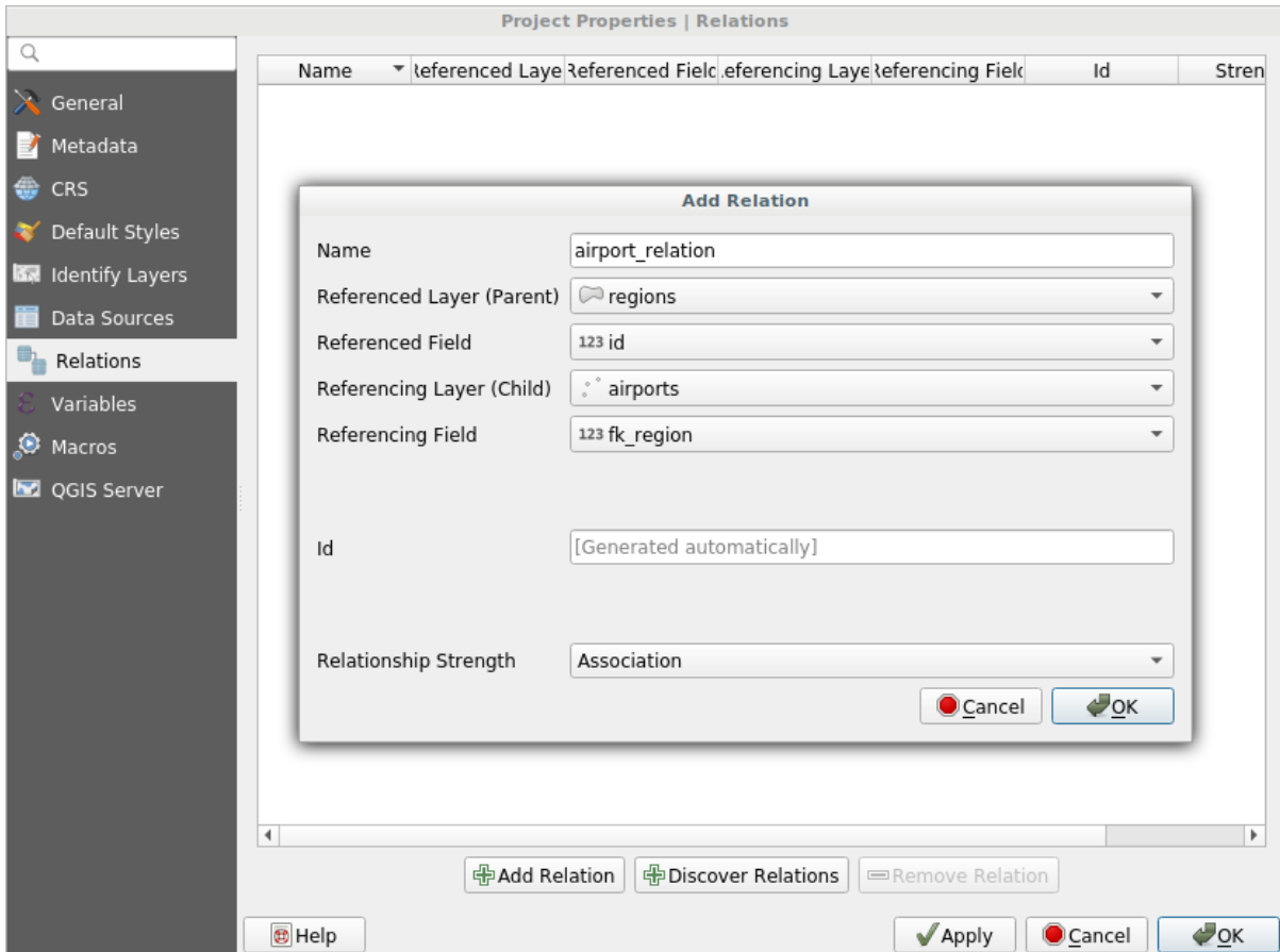
Рис. 13.85: Relation Manager
