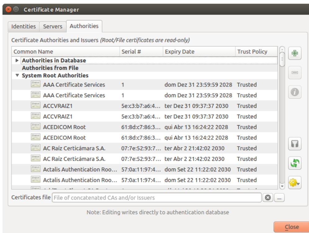
Рис. 19.24: Authorities editor
