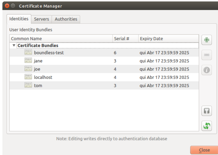
Рис. 19.29: Identities editor
