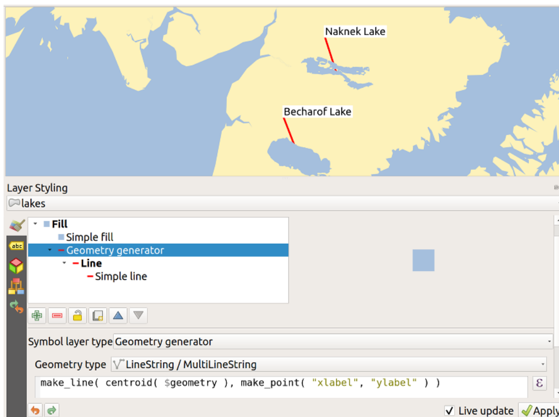
Рис. 13.43: Moved labels
