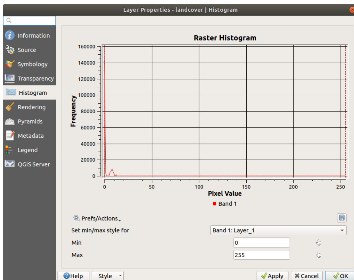
Рис. 14.10: Raster Histogram
