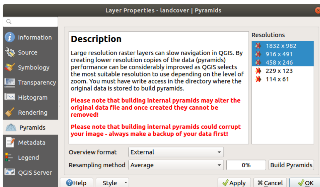
Рис. 14.12: Raster Pyramids
