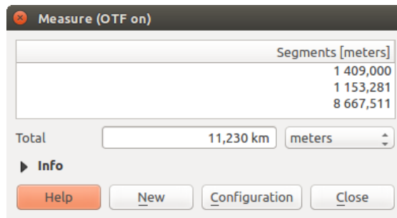
Рис. 11.14: Measure Distance
