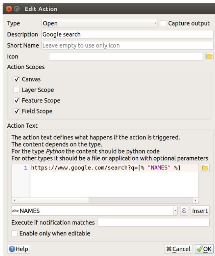
Рис. 13.65: Edit action dialog configured with the example
