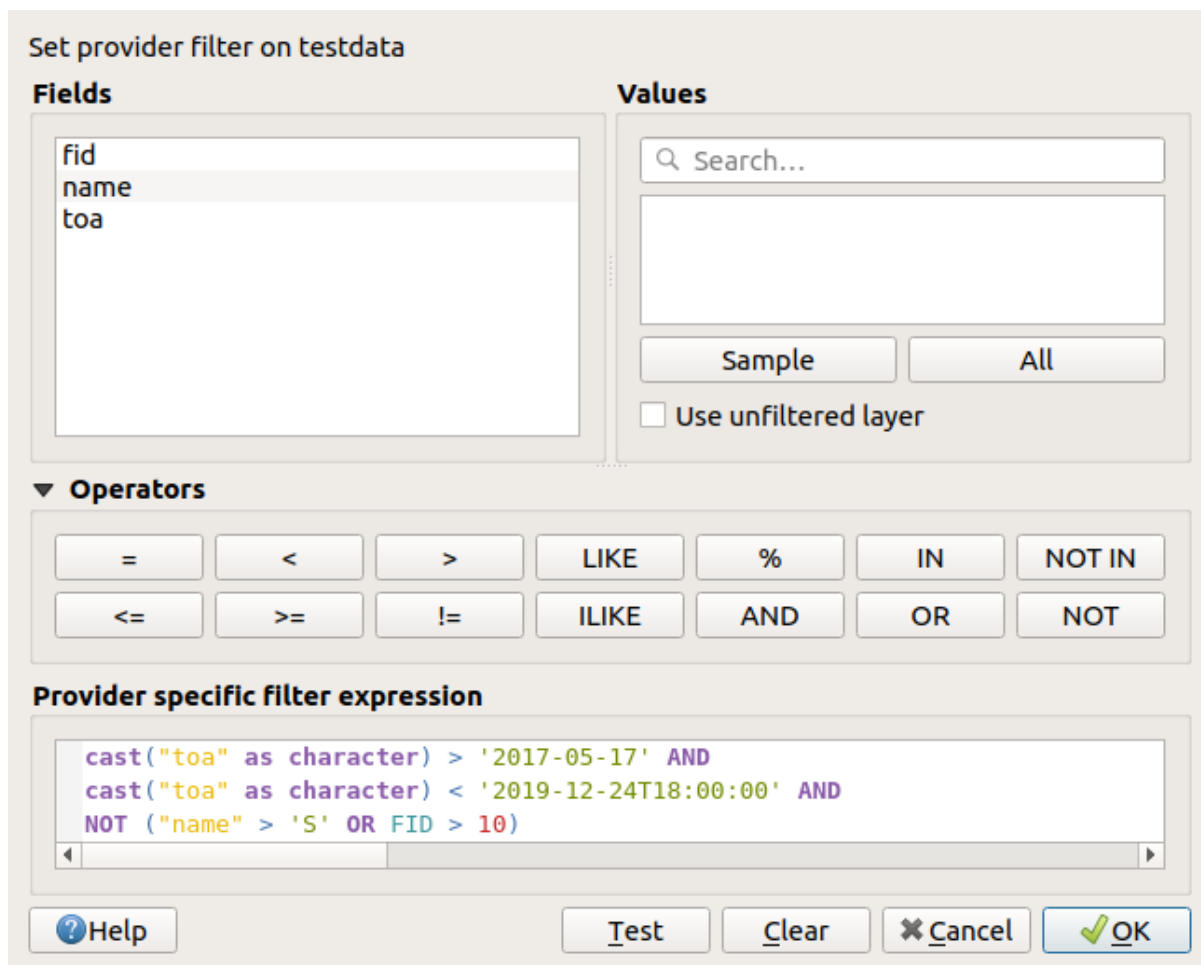
Рис. 13.9: Query Builder
