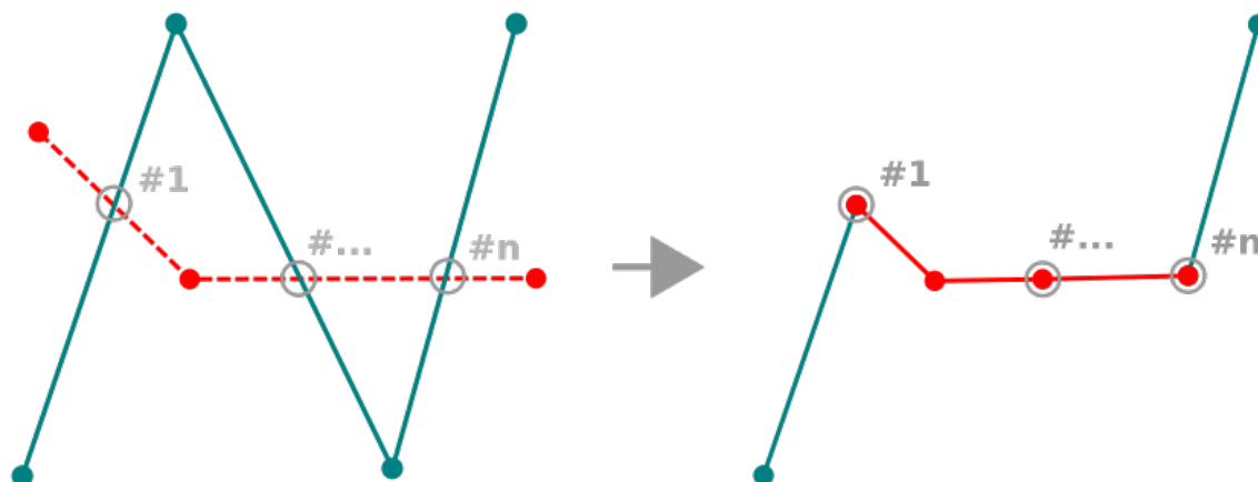
Рис. 13.98: Reshape line
