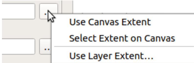
Рис. 21.11: Extent selector
