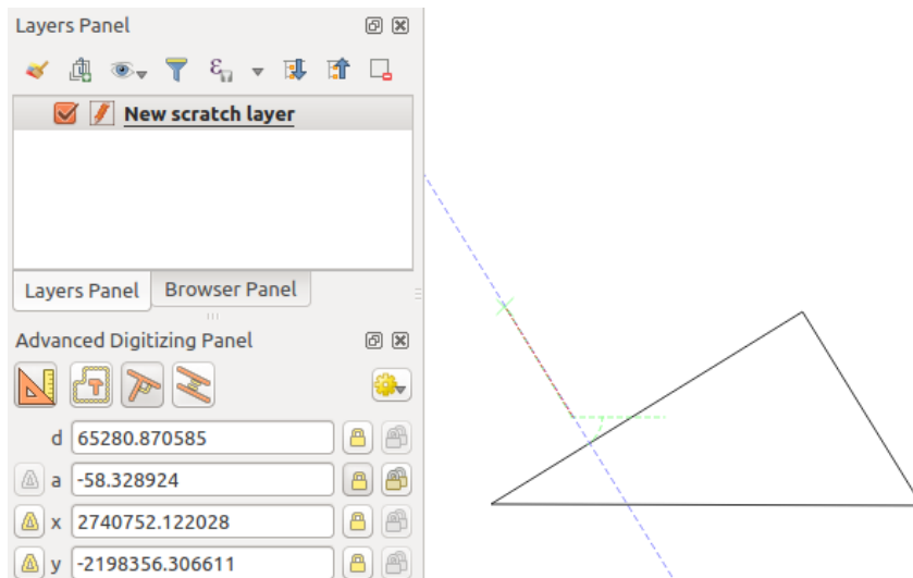
Рис. 13.105: Perpendicular digitizing
