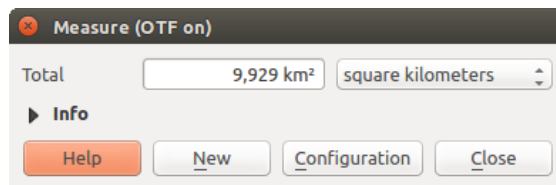
Рис. 11.15: Measure Area
