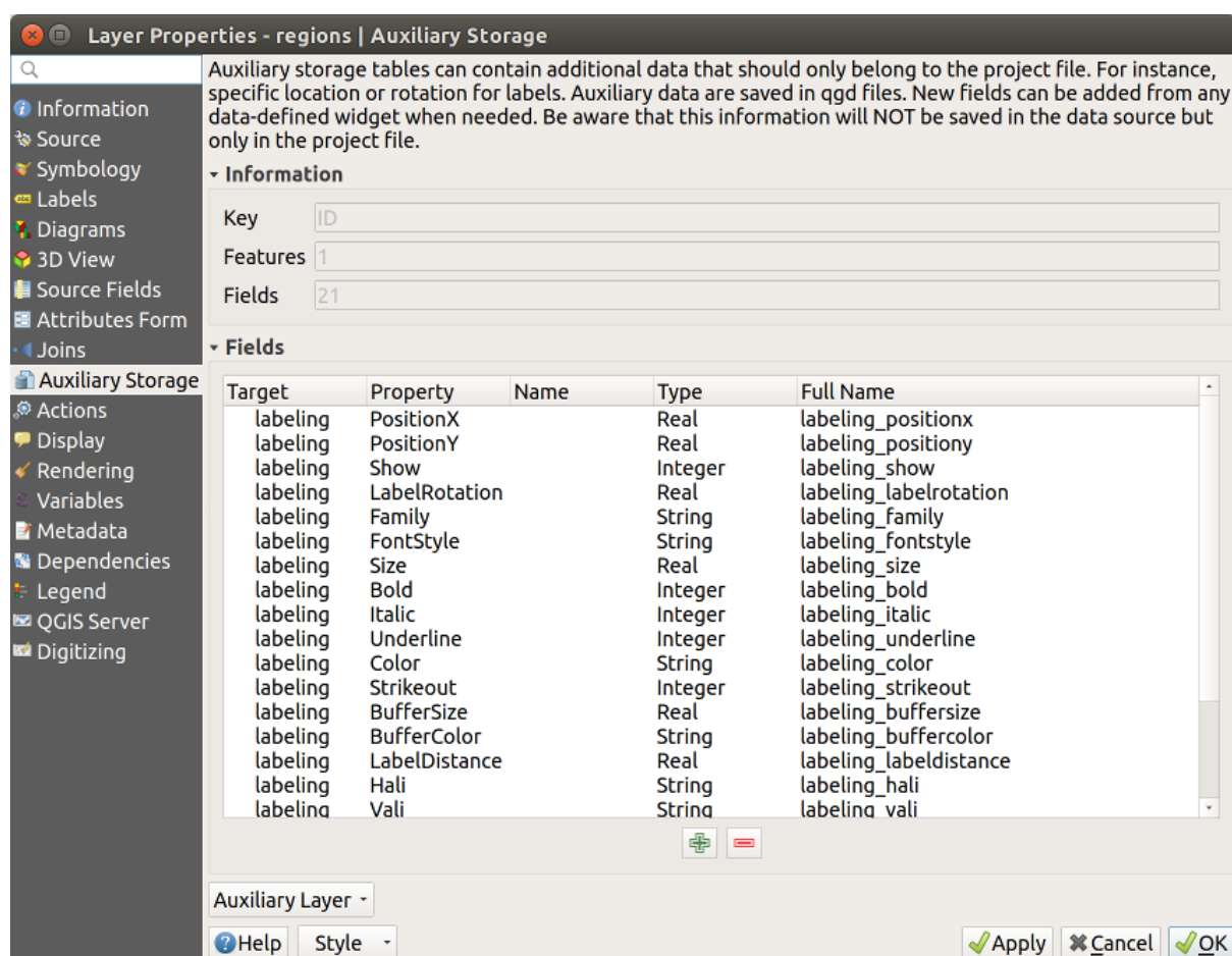
Рис. 13.57: Auxiliary Fields
