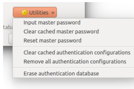
Рис. 19.15: Utilities menu
