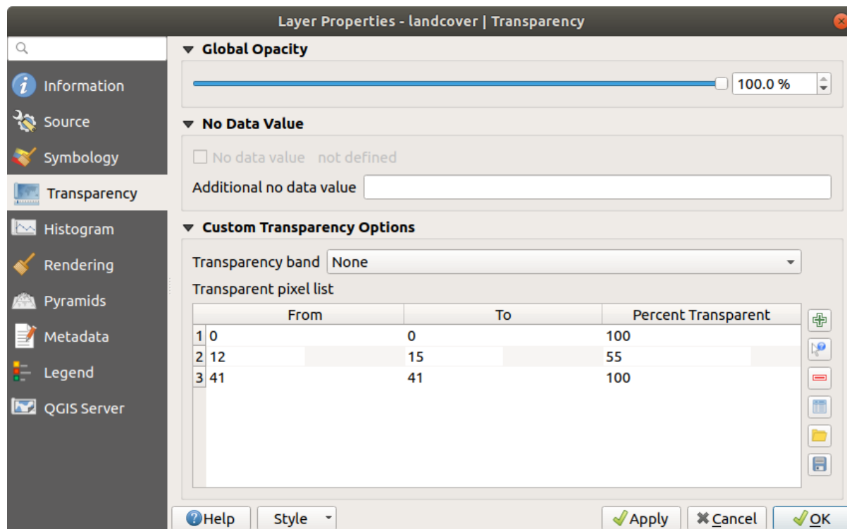
Рис. 14.9: Raster Transparency
