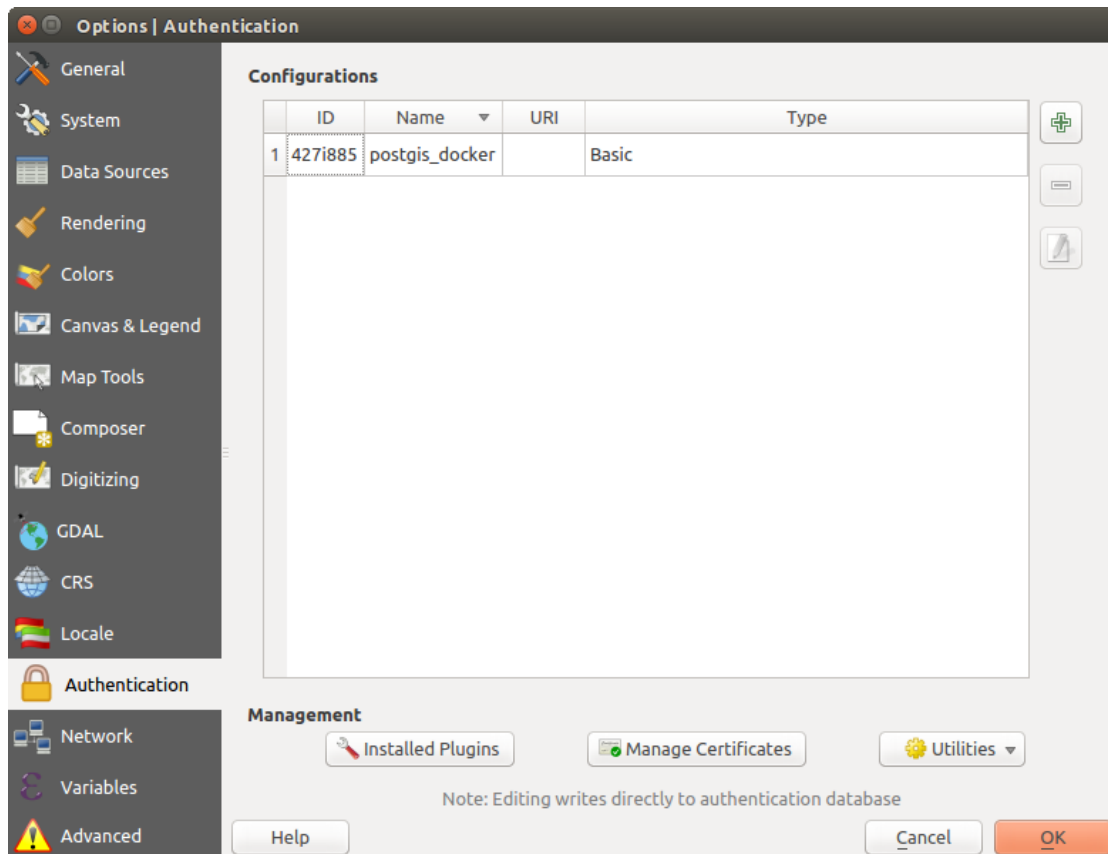
Рис. 19.5: Configurations editor
