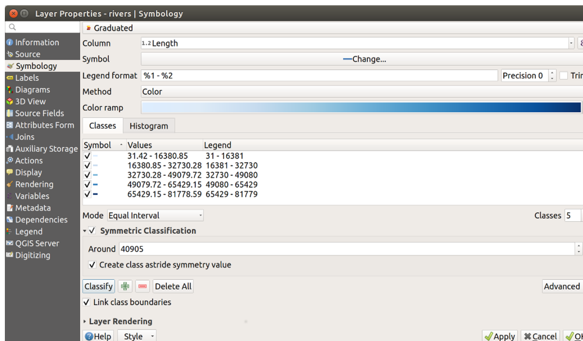
Рис. 13.12: Graduated Symbolizing options
