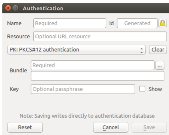
Рис. 19.13: PKI PKCS#12 file paths authentication configs
