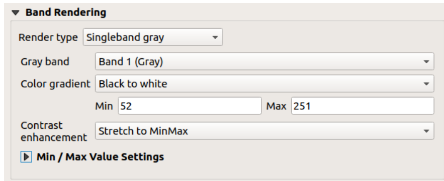
Рис. 14.4: Raster Symbology - Singleband gray rendering
