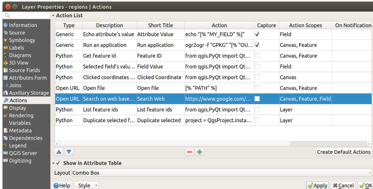
Gambar. 13.64: Overview action dialog with some sample actions
