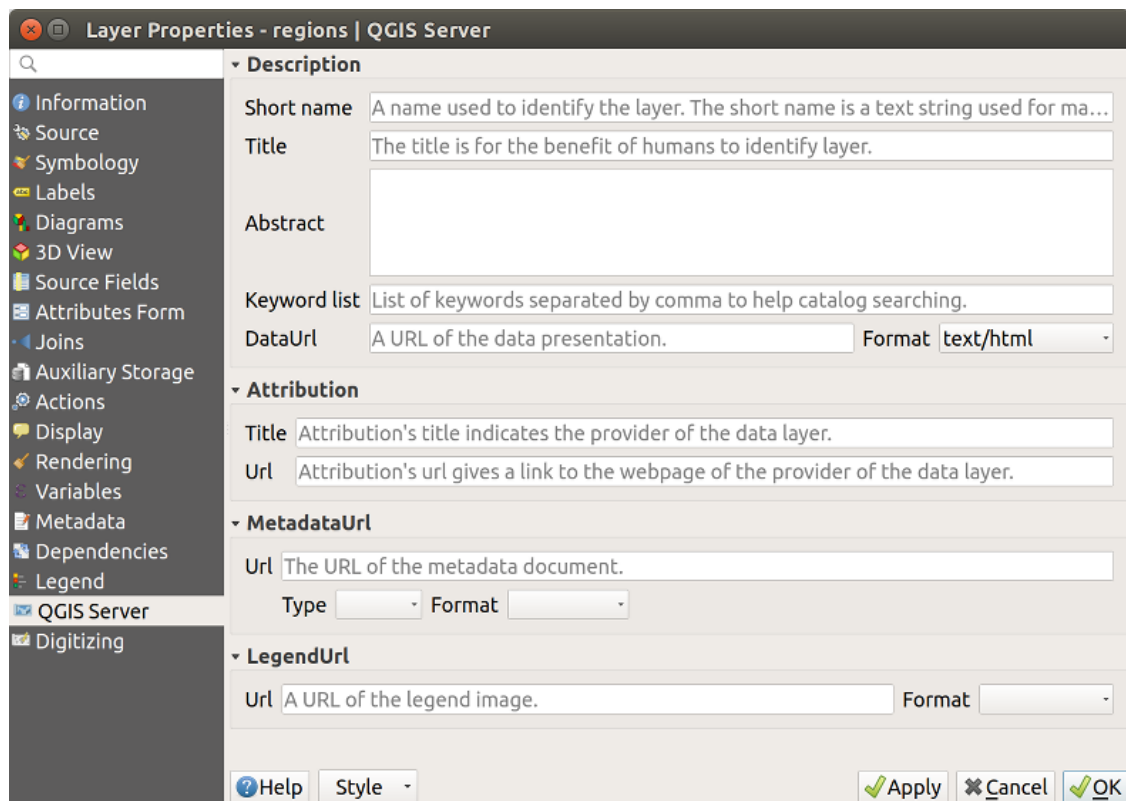
Gambar. 13.71: QGIS Server tab in vector layers properties dialog
