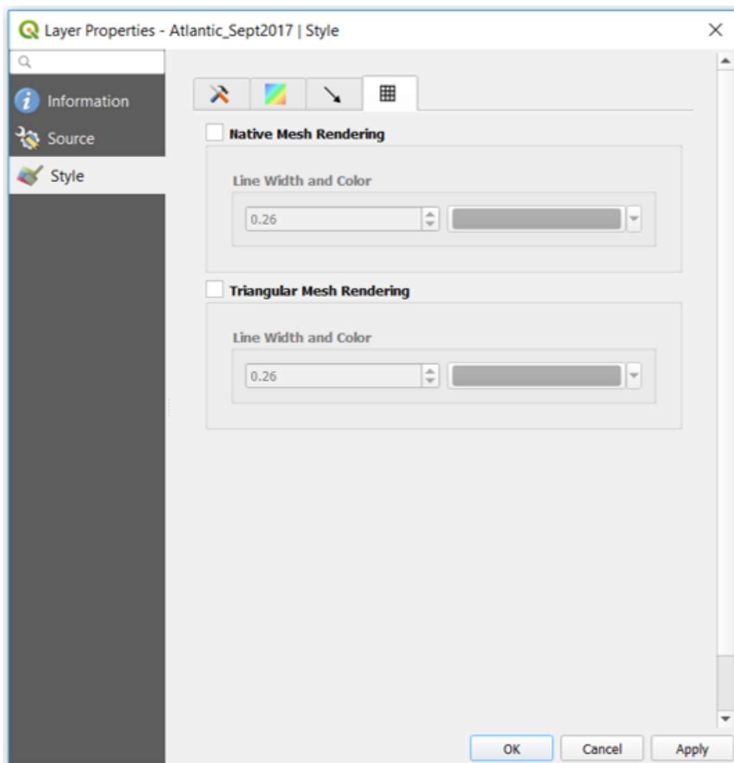
Gambar. 15.10: Mesh Rendering
