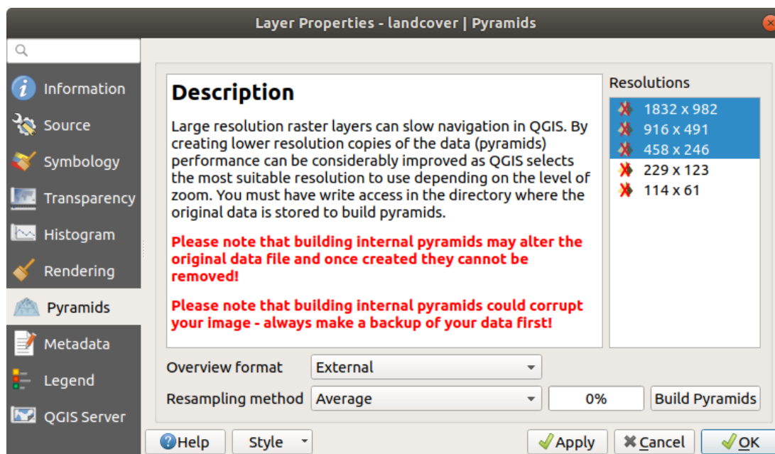
Gambar. 14.12: Raster Pyramids
