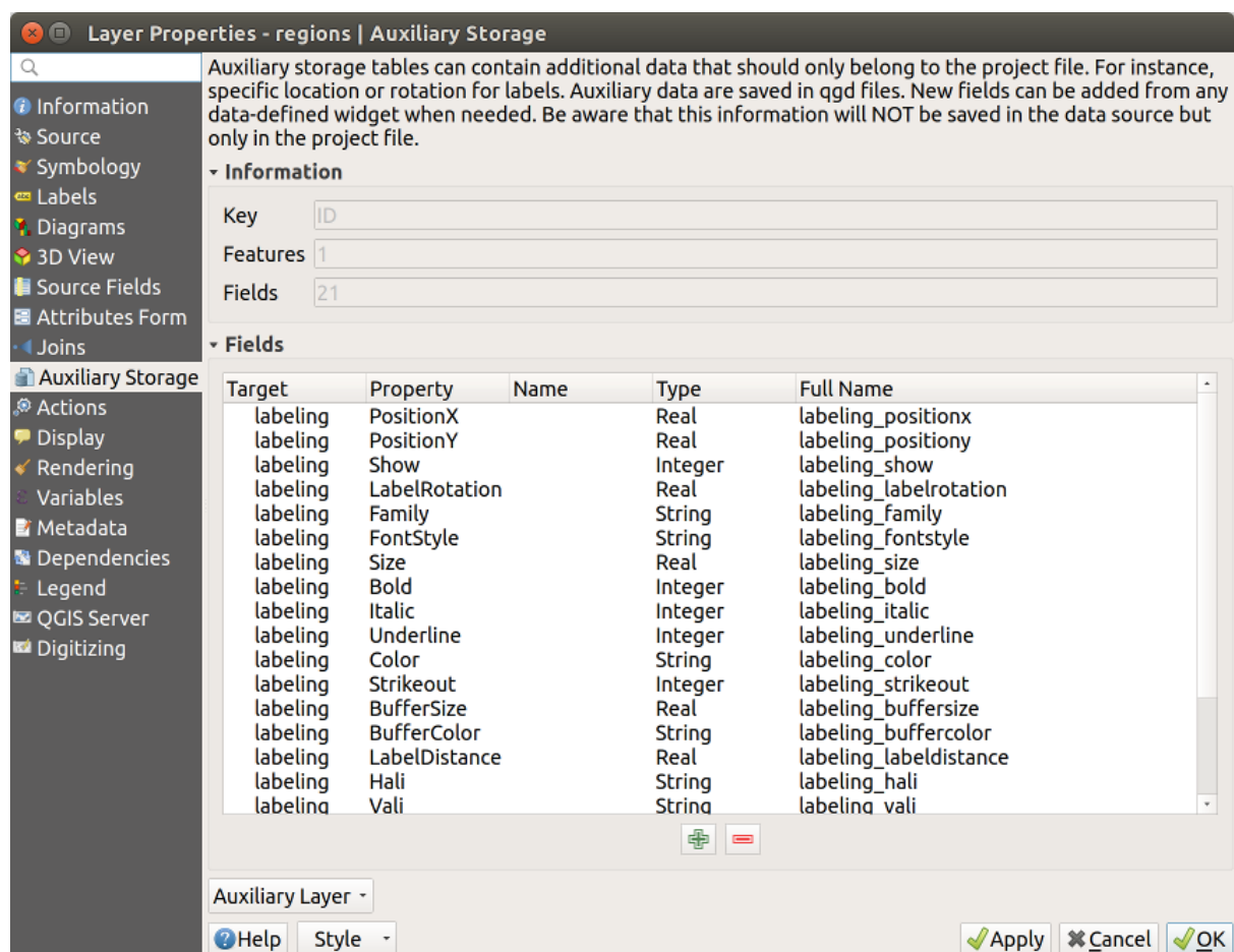
Gambar. 13.57: Auxiliary Fields
