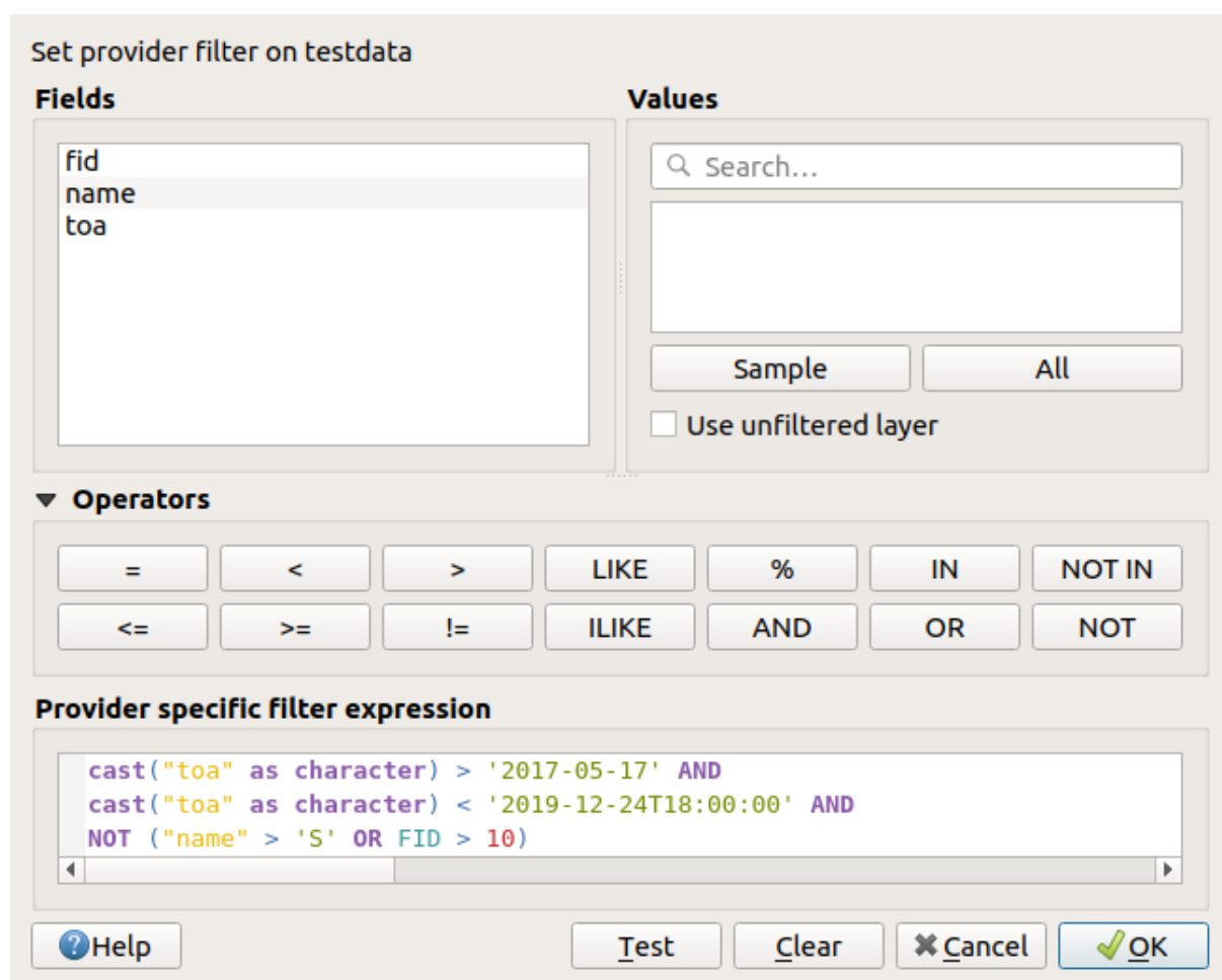
Gambar. 13.9: Query Builder
