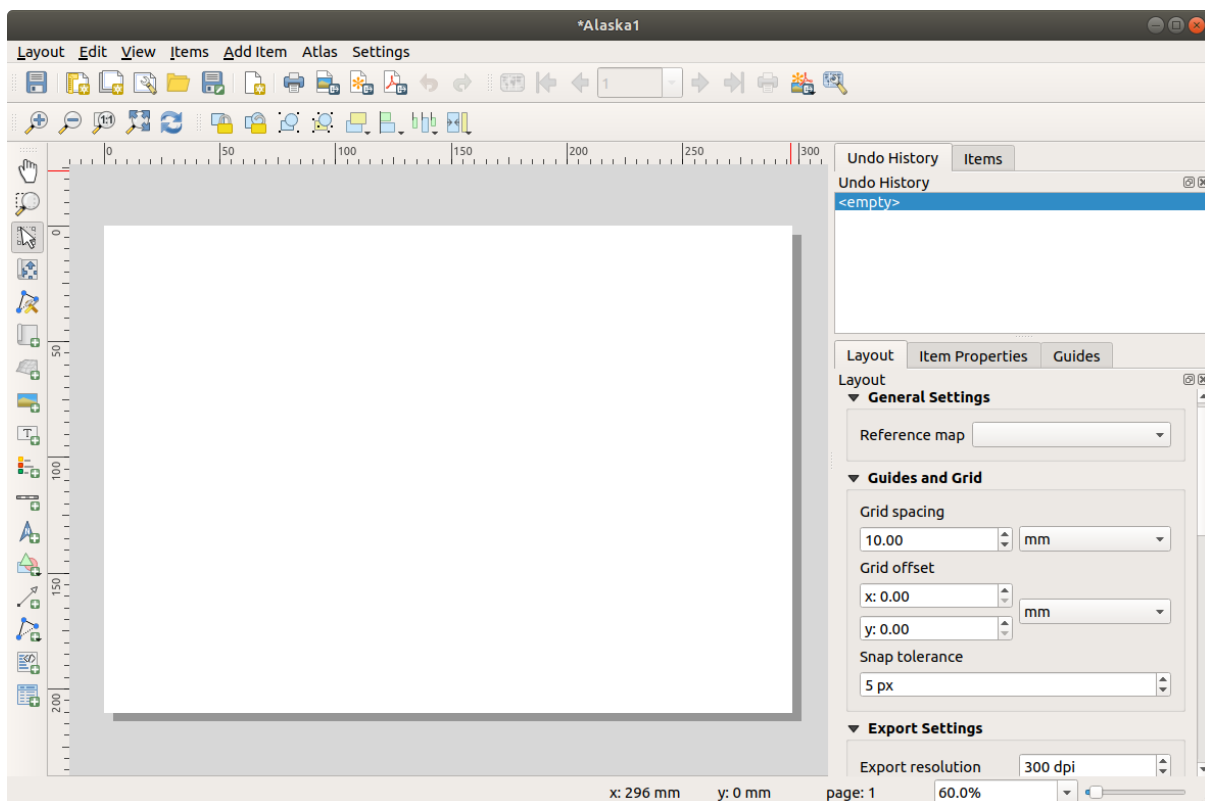
Gambar. 16.2: Print Layout
