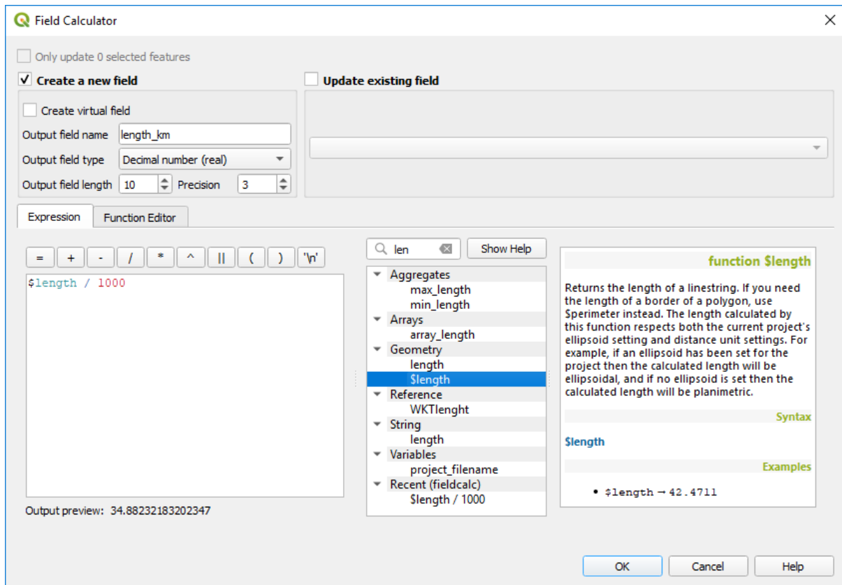
Gambar. 13.81: Field Calculator
