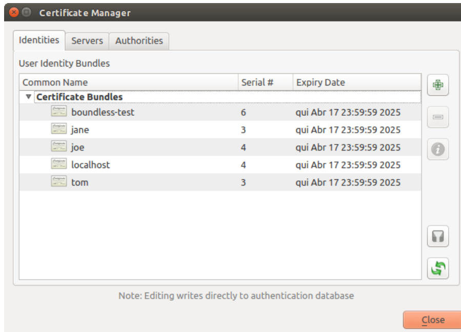
Gambar. 19.29: Identities editor
