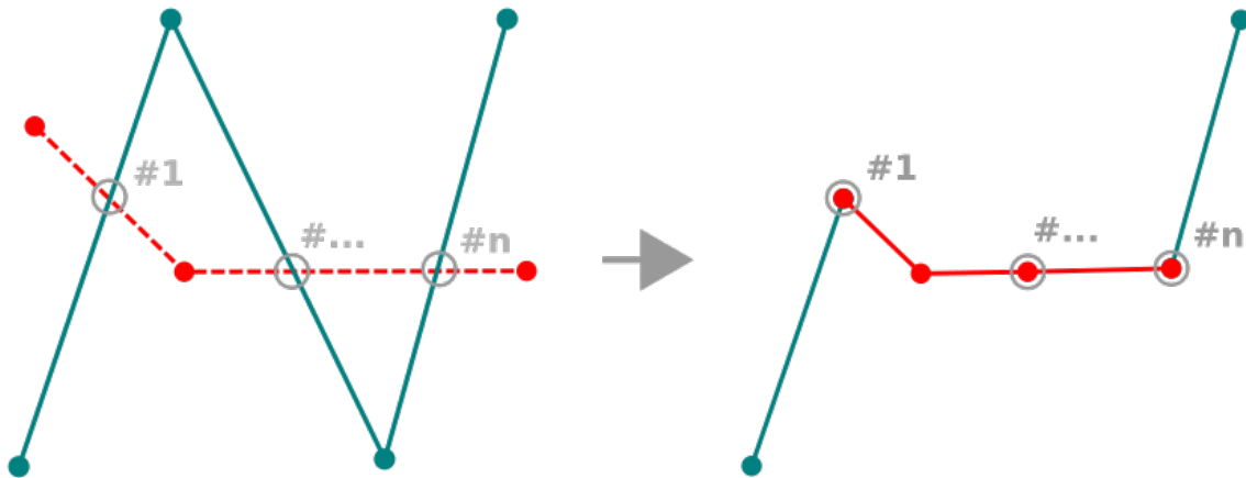
Gambar. 13.98: Reshape line
