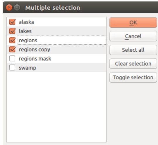
Gambar. 21.14: Multiple Selection
