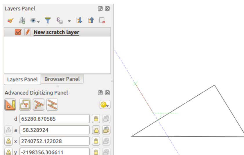
Gambar. 13.105: Perpendicular digitizing
