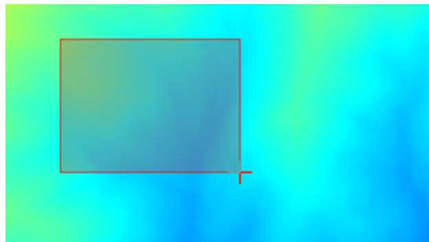
Gambar. 21.13: Extent Drag
