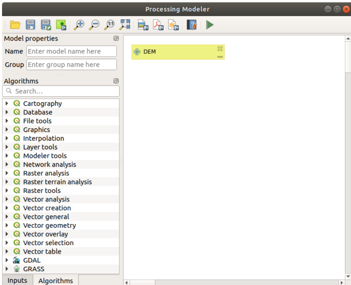
Gambar. 21.21: Model Inputs
