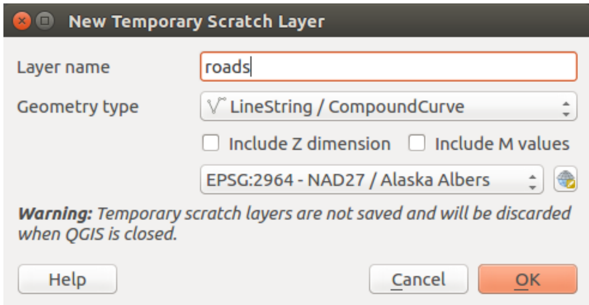
Gambar. 12.14: Creating a new Temporary Scratch layer dialog
