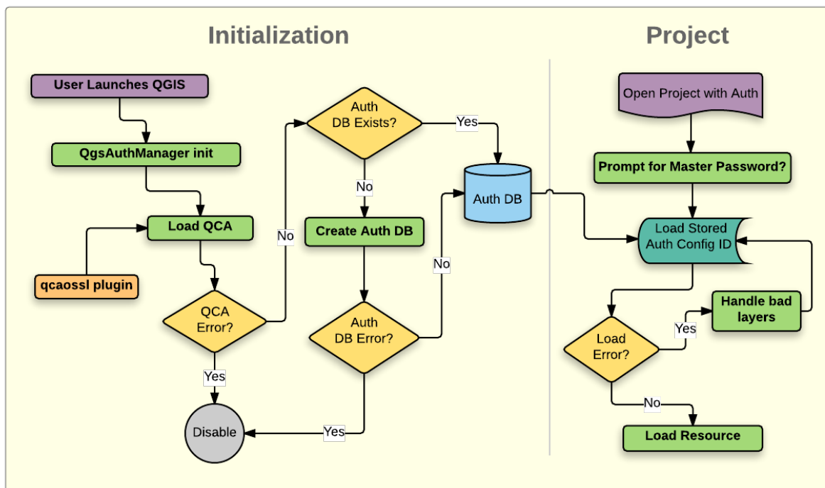
Gambar. 19.1: Anatomy of authentication system
