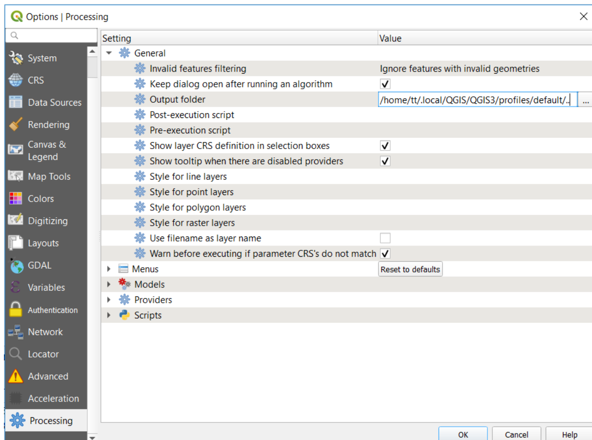
Gambar. 9.18: Processing Settings tab in QGIS
