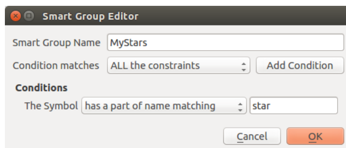
Gambar. 13.2: Creating a Smart Group
