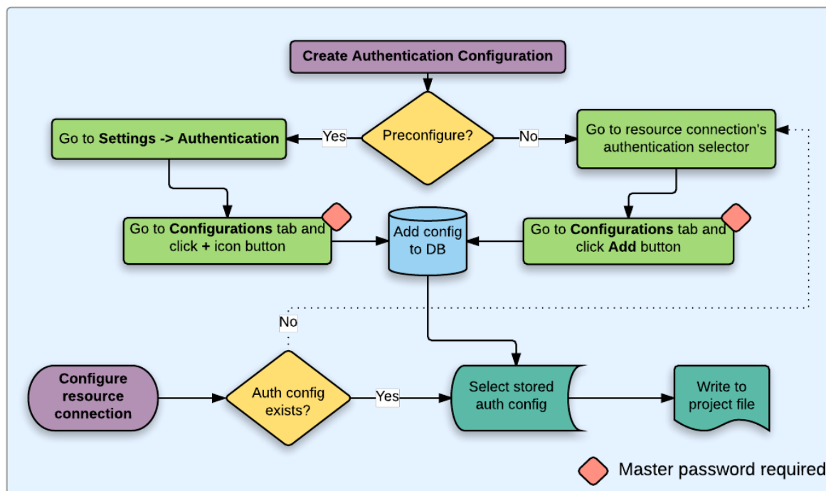
Gambar. 19.19: Generic user workflow
