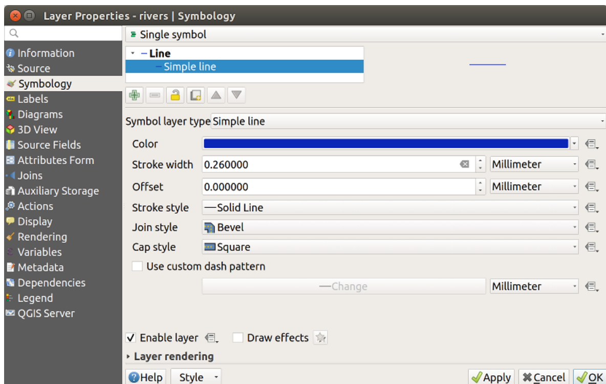
Gambar. 13.10: Single symbol line properties
