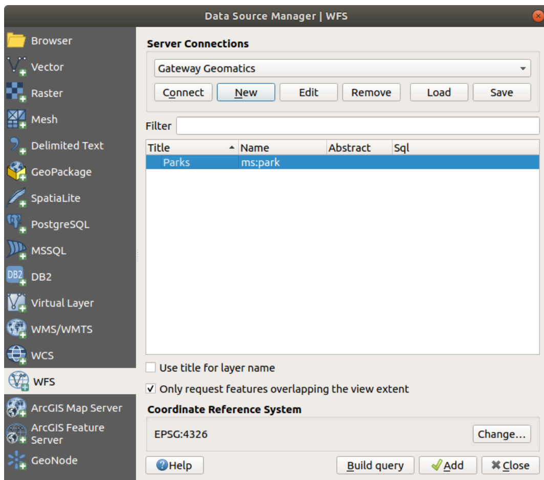
Gambar. 17.5: Adding a WFS layer
