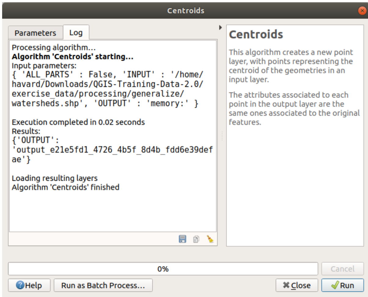
Gambar. 21.16: Algorithm Dialog - Log
