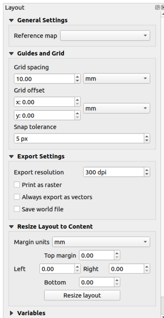
Gambar. 16.3: Layout Settings in the Print Layout
