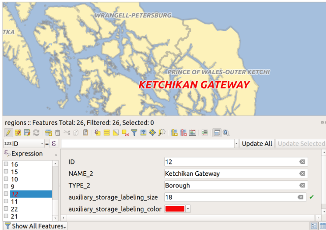
Gambar. 13.62: Form with auxiliary fields
