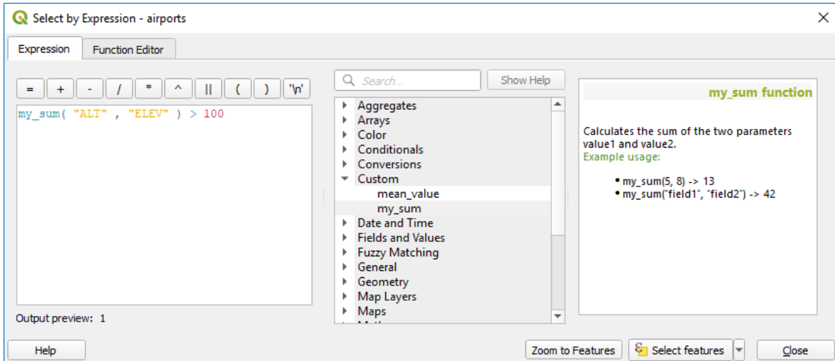
Gambar. 13.75: Custom Function added to the Expression tab
