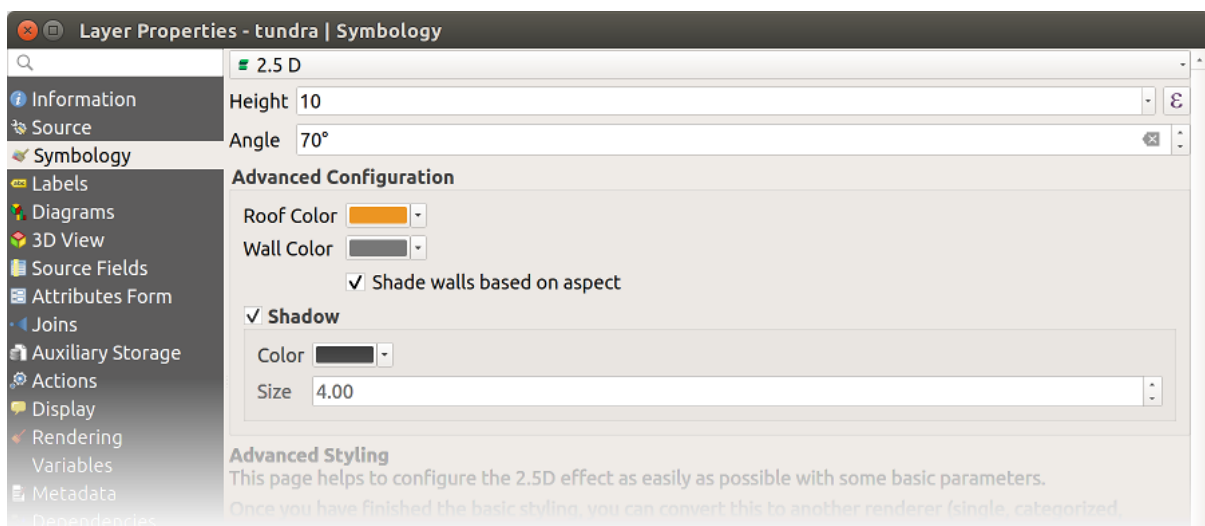
Gambar. 13.20: 2.5D dialog
