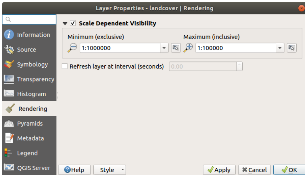
Gambar. 14.11: Raster Rendering
