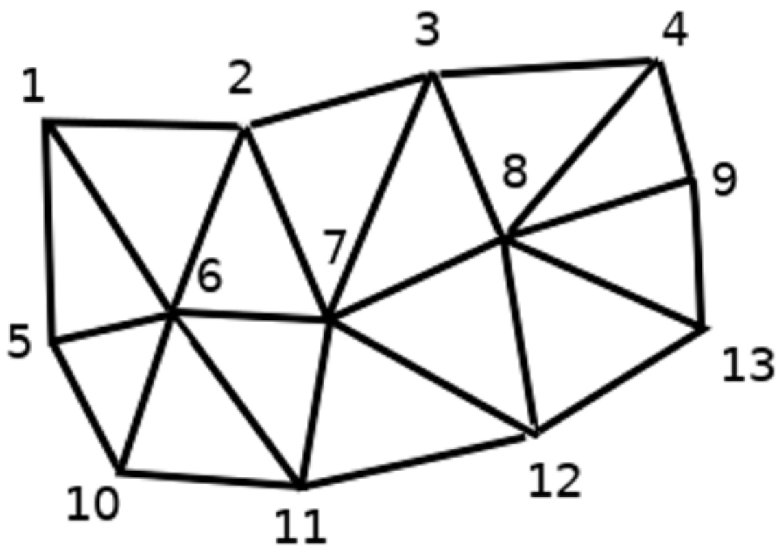
Gambar. 15.2: Triangular grid with numbered vertices
