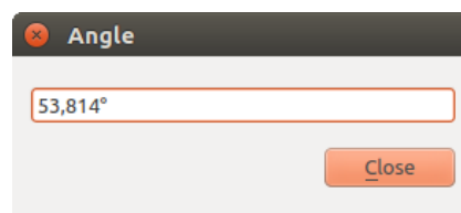
Gambar. 11.16: Measure Angle
