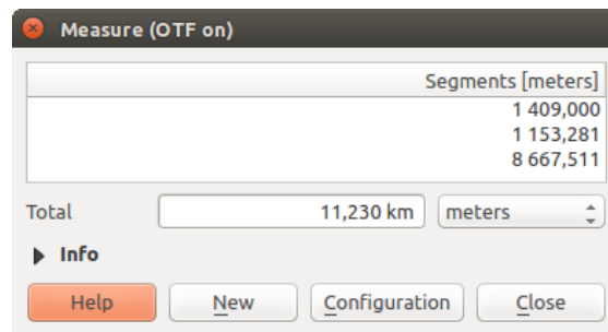
Gambar. 11.14: Measure Distance
