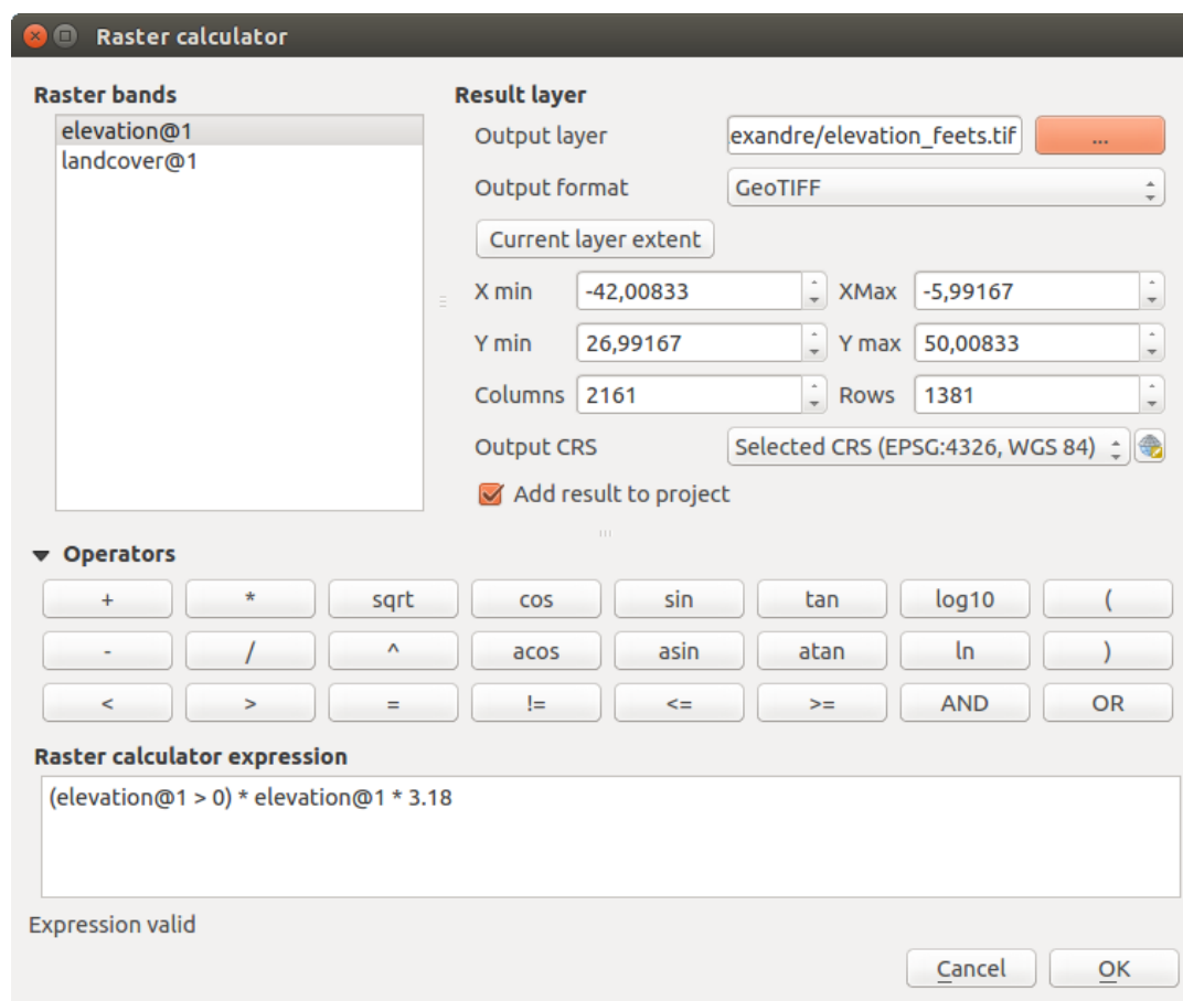
Gambar. 14.14: Raster Calculator
