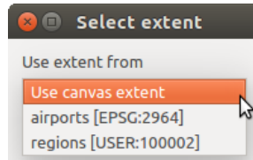
Gambar. 21.12: Extent List
