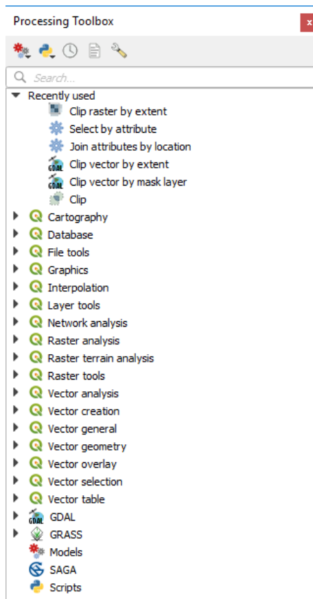
Gambar. 21.6: Processing Toolbox
