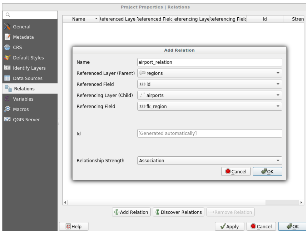
Gambar. 13.85: Relation Manager
