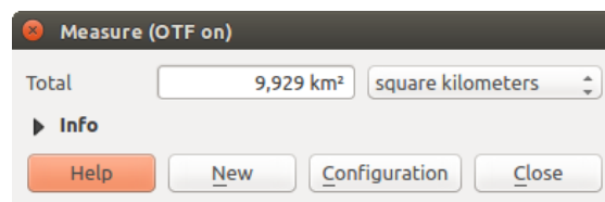
Gambar. 11.15: Measure Area
