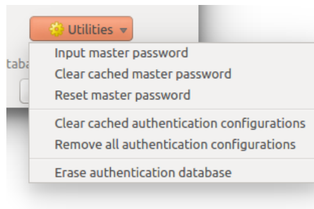
Gambar. 19.15: Utilities menu
