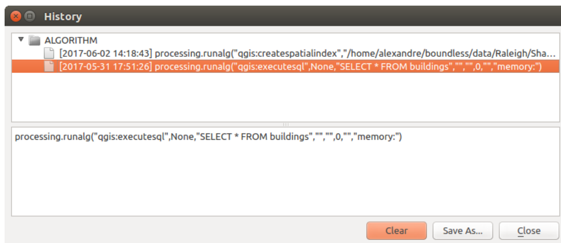
Gambar. 21.17: History
