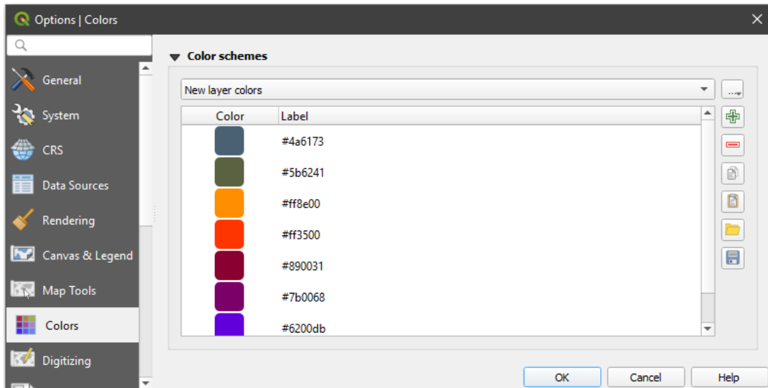
Gambar. 9.7: Colors Settings
