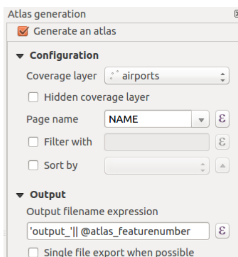
Gambar. 16.57: Atlas Panel
