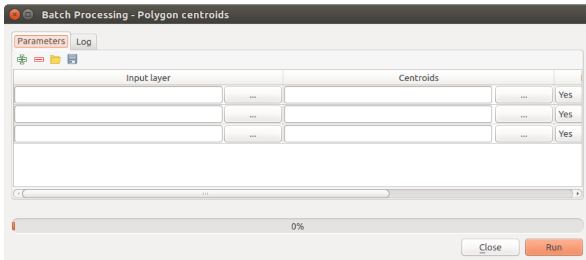
Gambar. 21.30: Batch Processing
