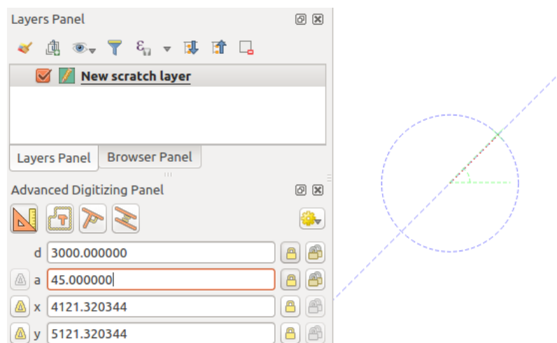
Gambar. 13.104: Fixed angle segment
