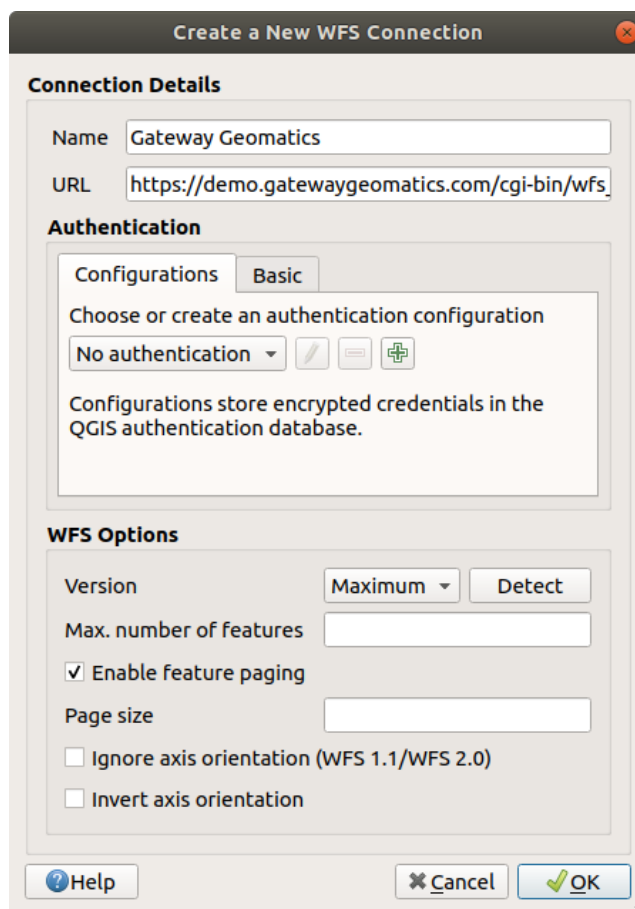
Gambar. 17.4: Creating a connection to a WFS server
