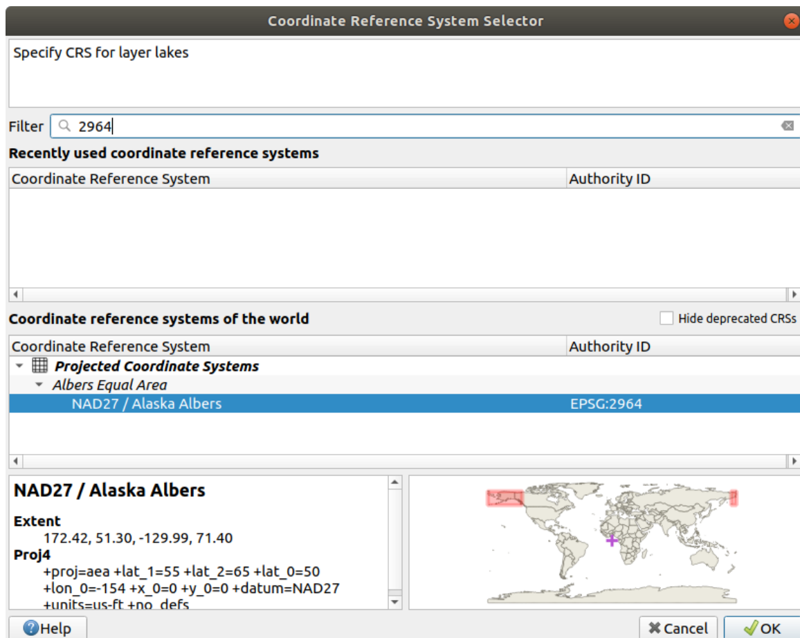
Gambar. 6.2: Select the Coordinate Reference System of data
