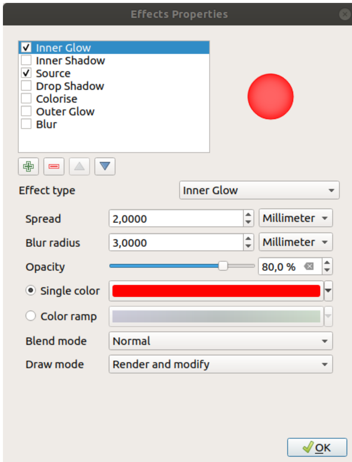
Figure 13.30: Draw Effects: Inner Glow dialog
