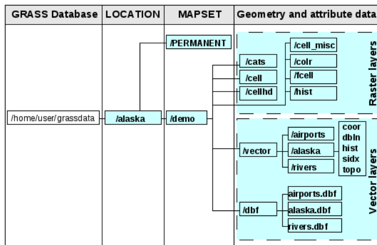
Figure 20.1: GRASS data in the alaska LOCATION
