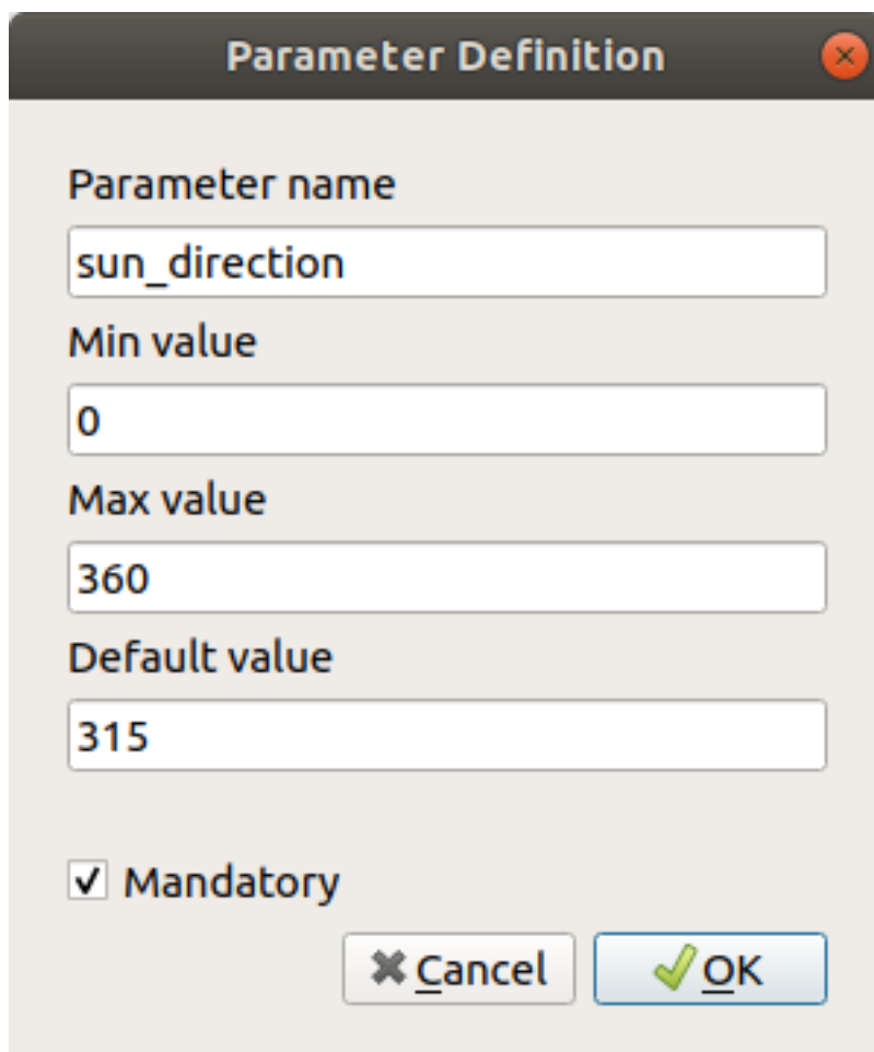
Figure 21.19: Model Parameters Definition
