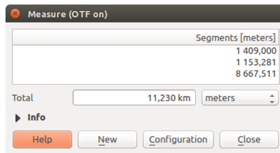
Figure 11.14: Measure Distance
