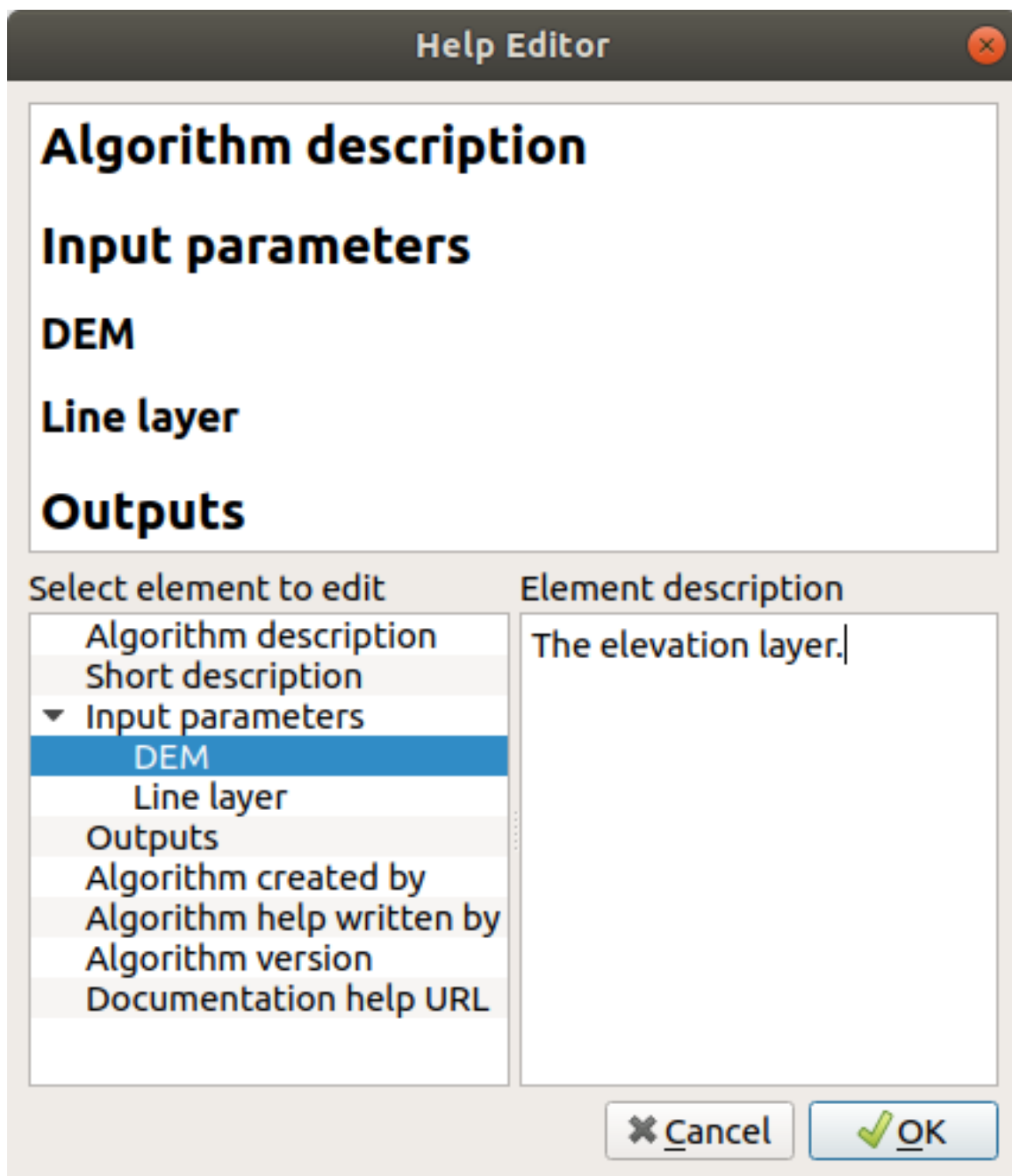
Figure 21.27: Editing Help
