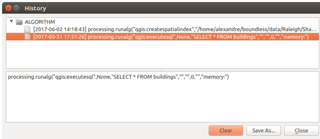
Figure 21.3: Processing History
