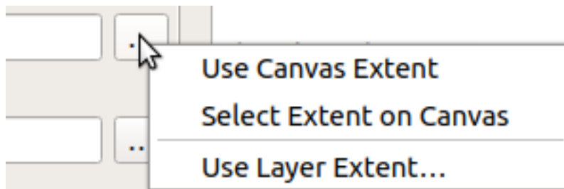
Figure 21.11: Extent selector
