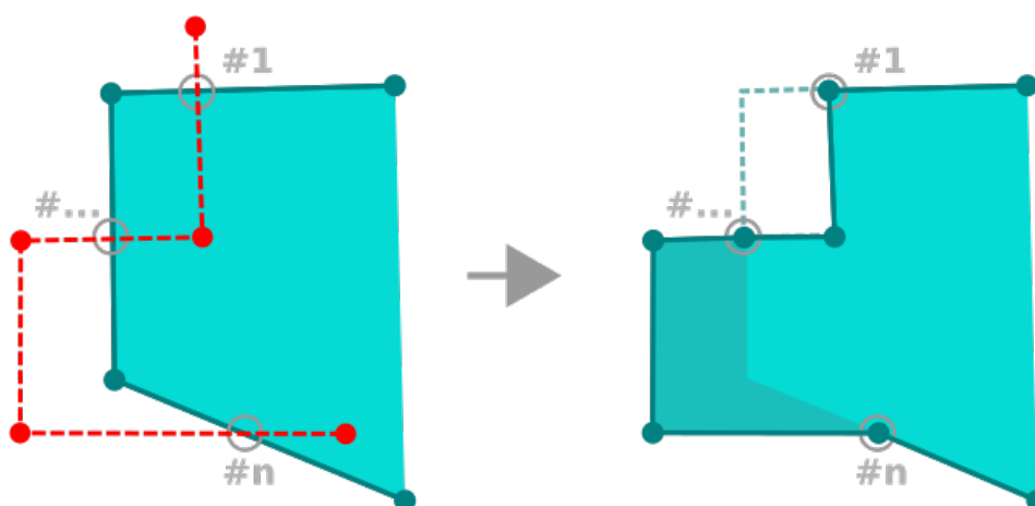
Figure 13.99: Remodelar polígono
