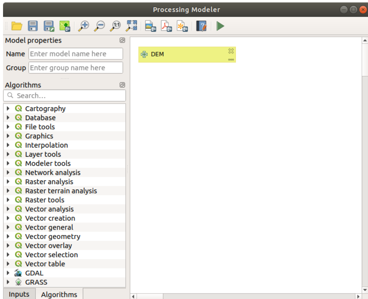
Figure 21.21: Model Inputs
