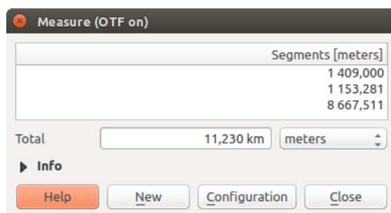
Figure 11.14: Medir Distancia
