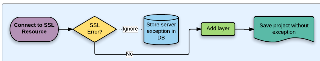
Figure 19.35: excepción de servidor SSL
