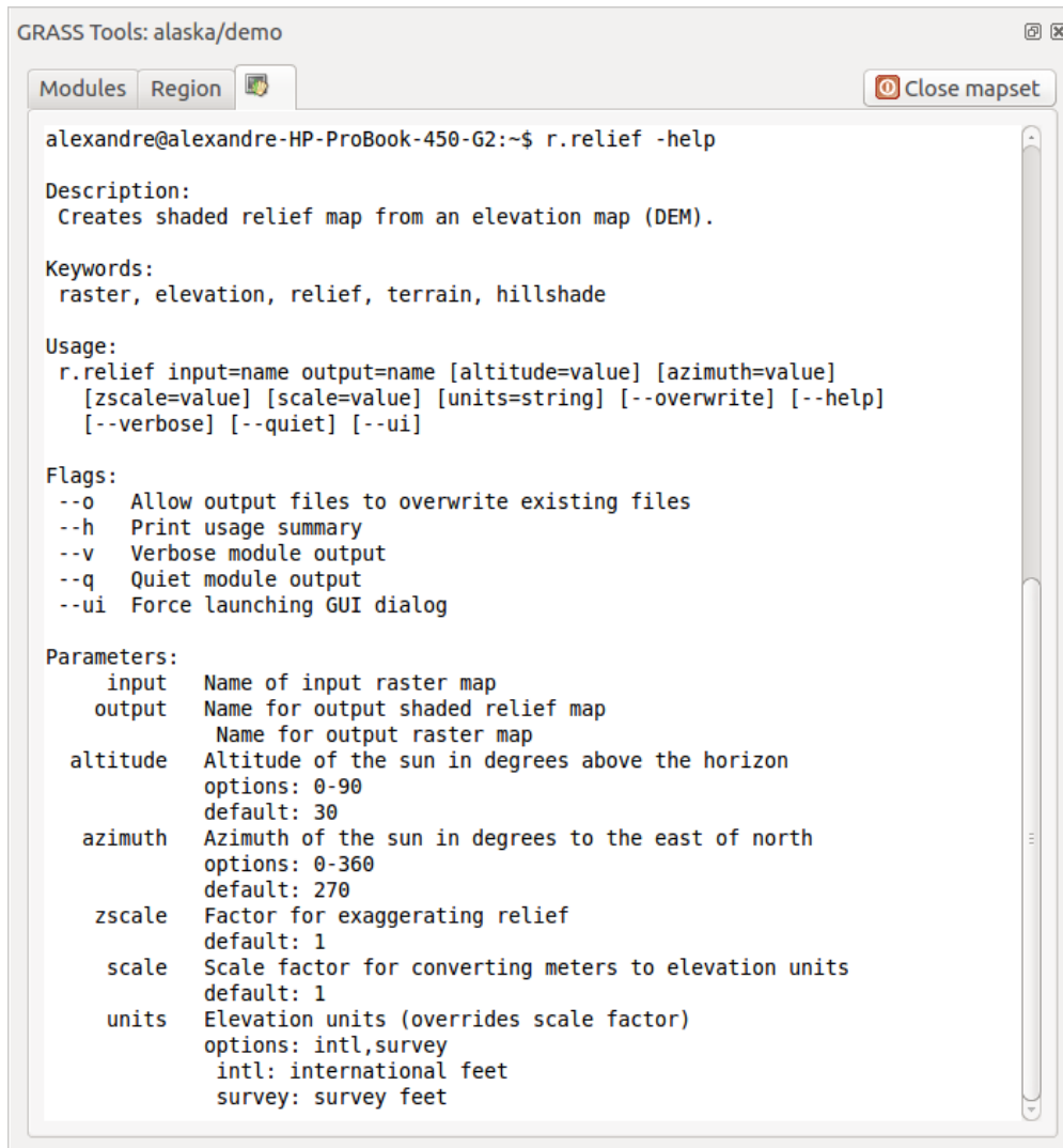
Figure 20.8: La consola de GRASS, módulo r.shaded.relief
