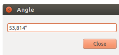
Figure 11.16: Medir Ángulo
