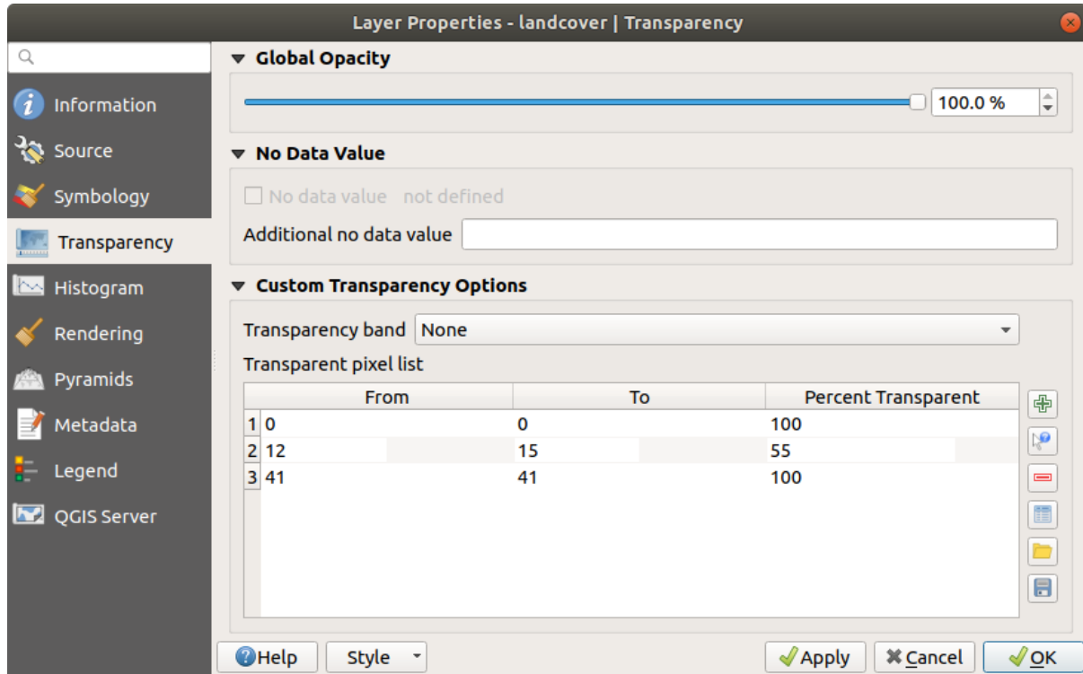
Figure 14.9: Raster Transparency
