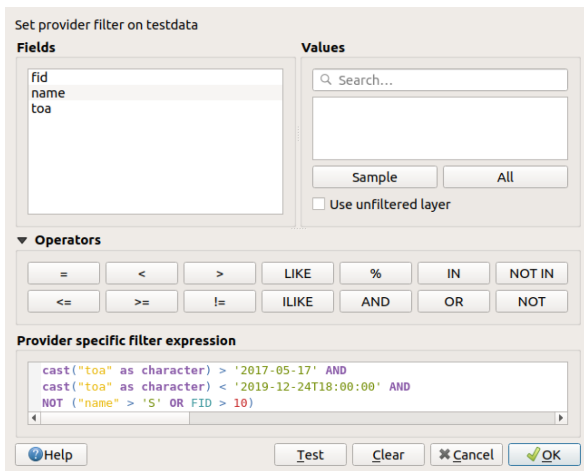
Figure 13.9: Constructor de Consulta
