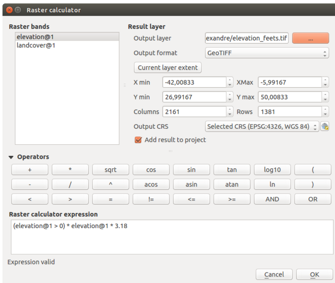
Figure 14.14: Calculadora Ráster
