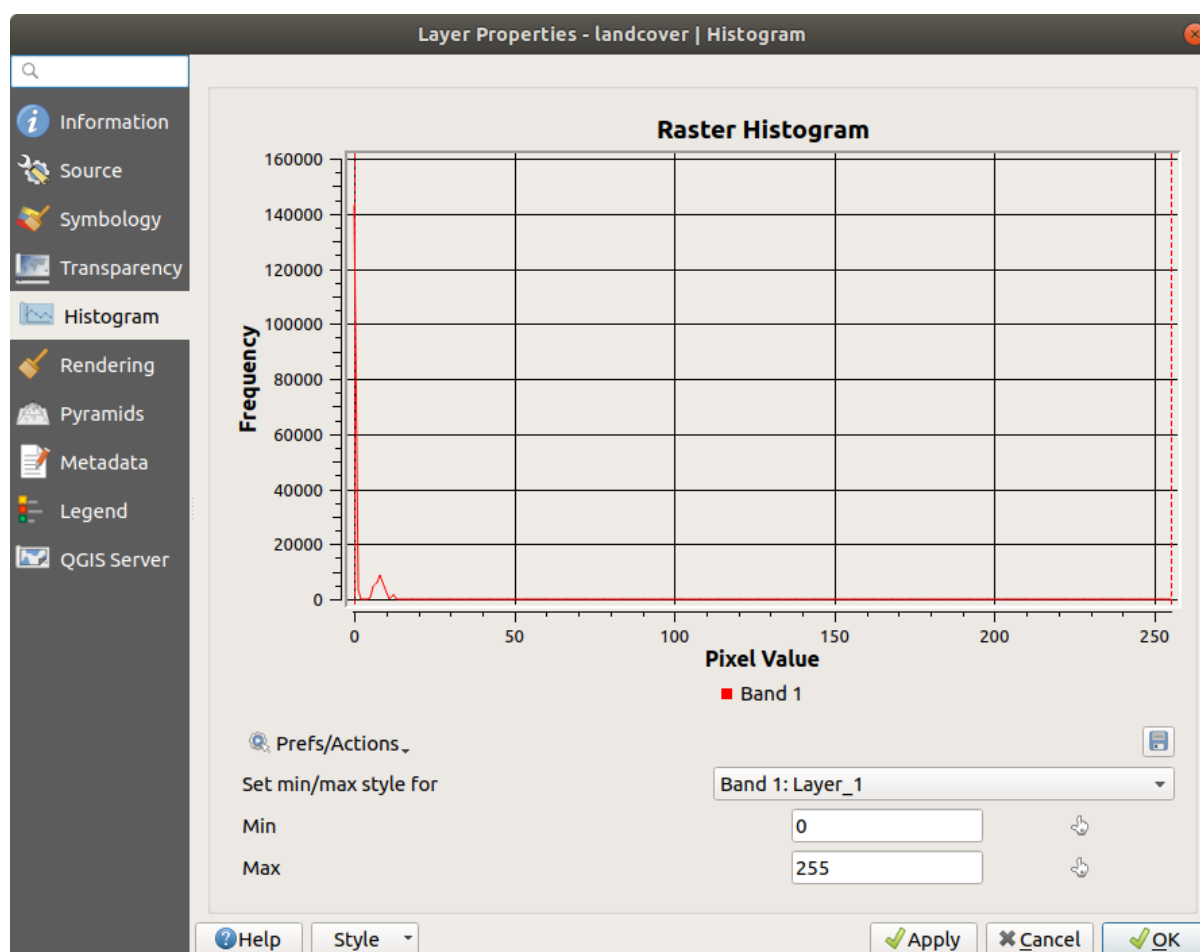
Figure 14.10: Raster Histogram
