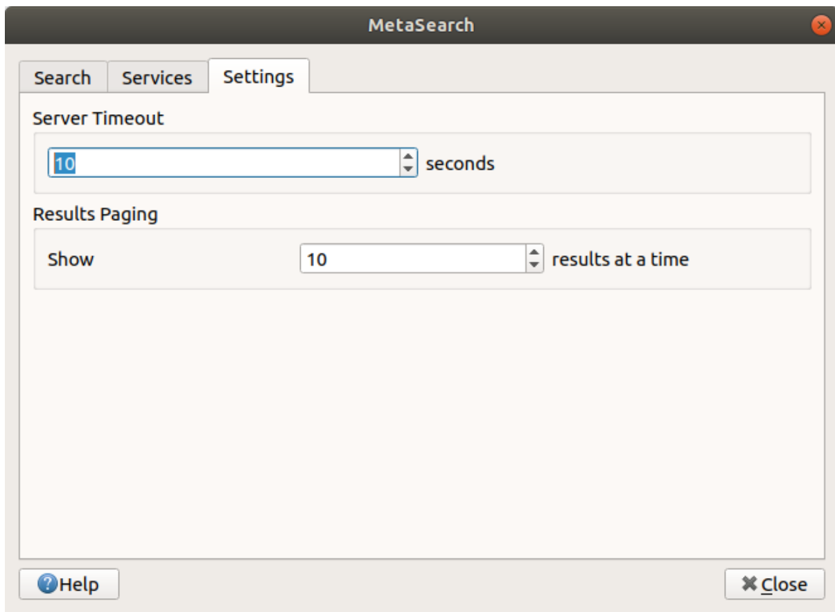
Figure 22.26: MetaSearch settings
