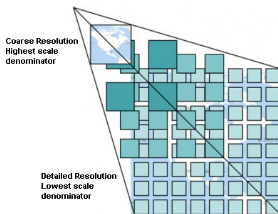
Figure 17.1: Concept of WMTS tile sets
