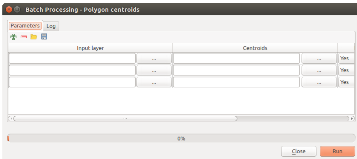
Figure 21.30: Batch Processing
