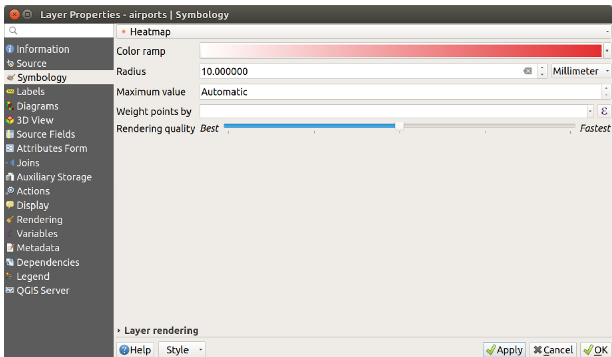
Figure 13.19: Heatmap dialog
