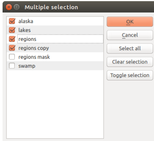
Figure 21.14: Multiple Selection
