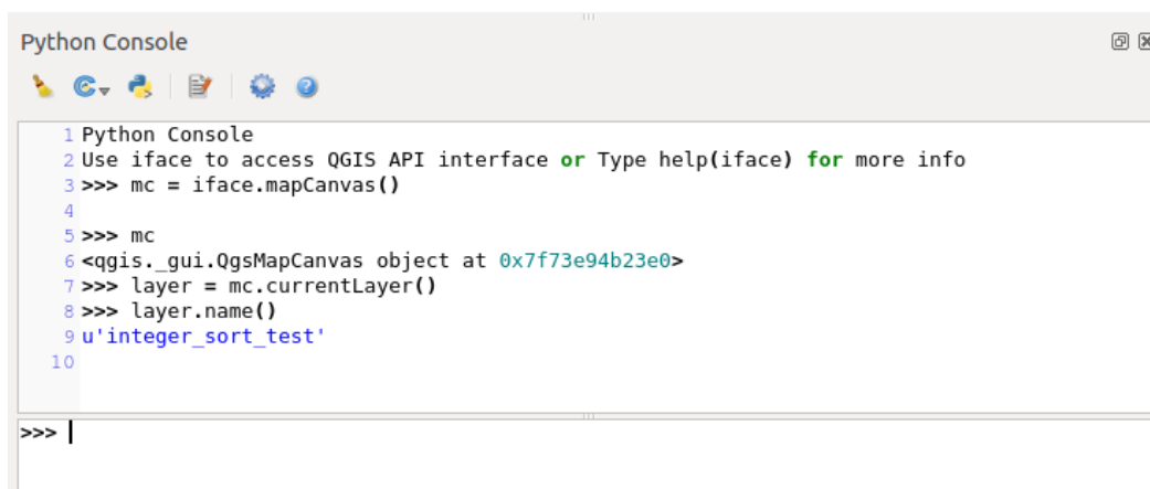
Figure 22.29: The Python Console
