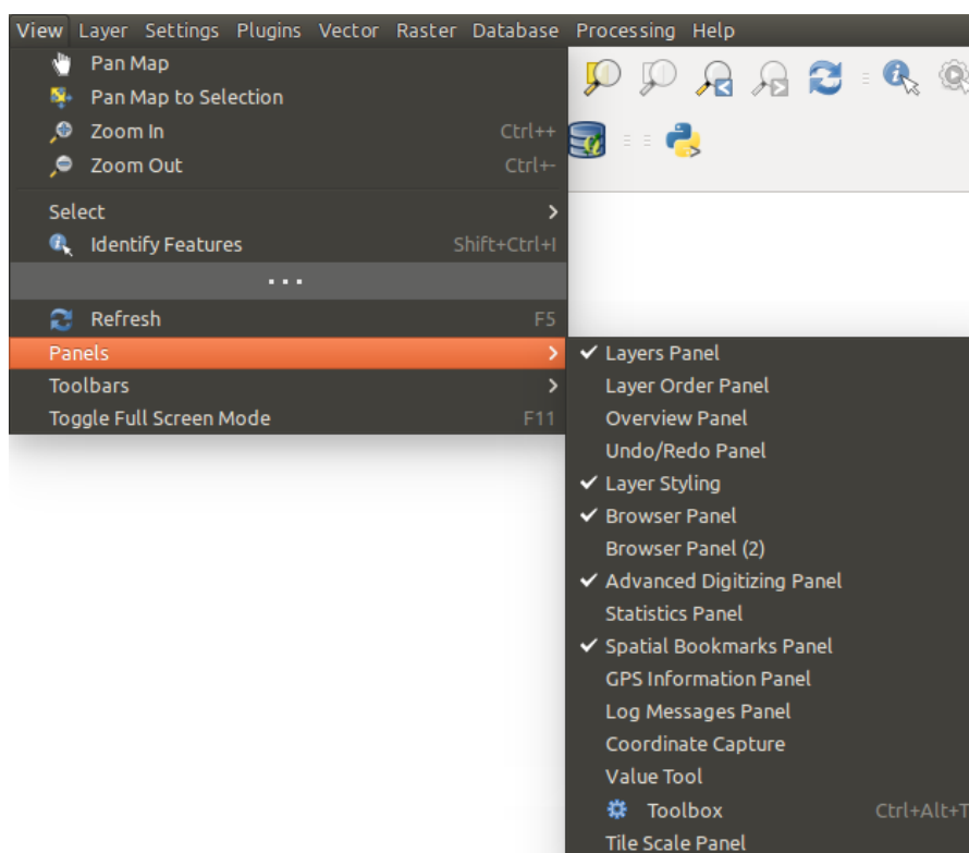
Figure 8.3: Panelové menu
