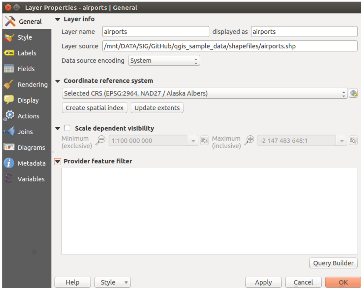
Figure 12.13: General menu in vector layers properties dialog
