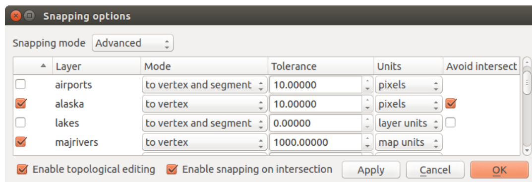
Figure 12.67: Edit snapping options on a layer basis (Advanced mode)
