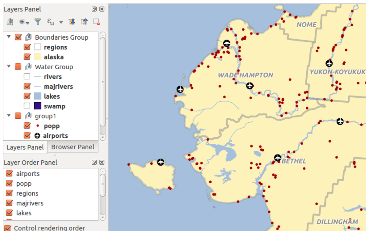
Gambar 7.4: Define a legend independent layer order
