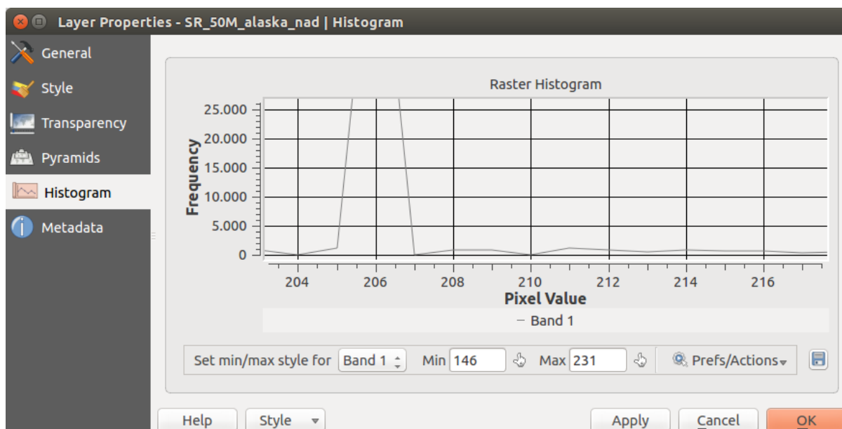
Gambar 13.8: Raster Histogram
