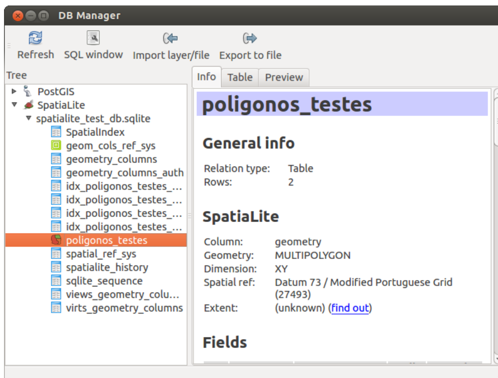
Gambar 20.7: DB Manager dialog
