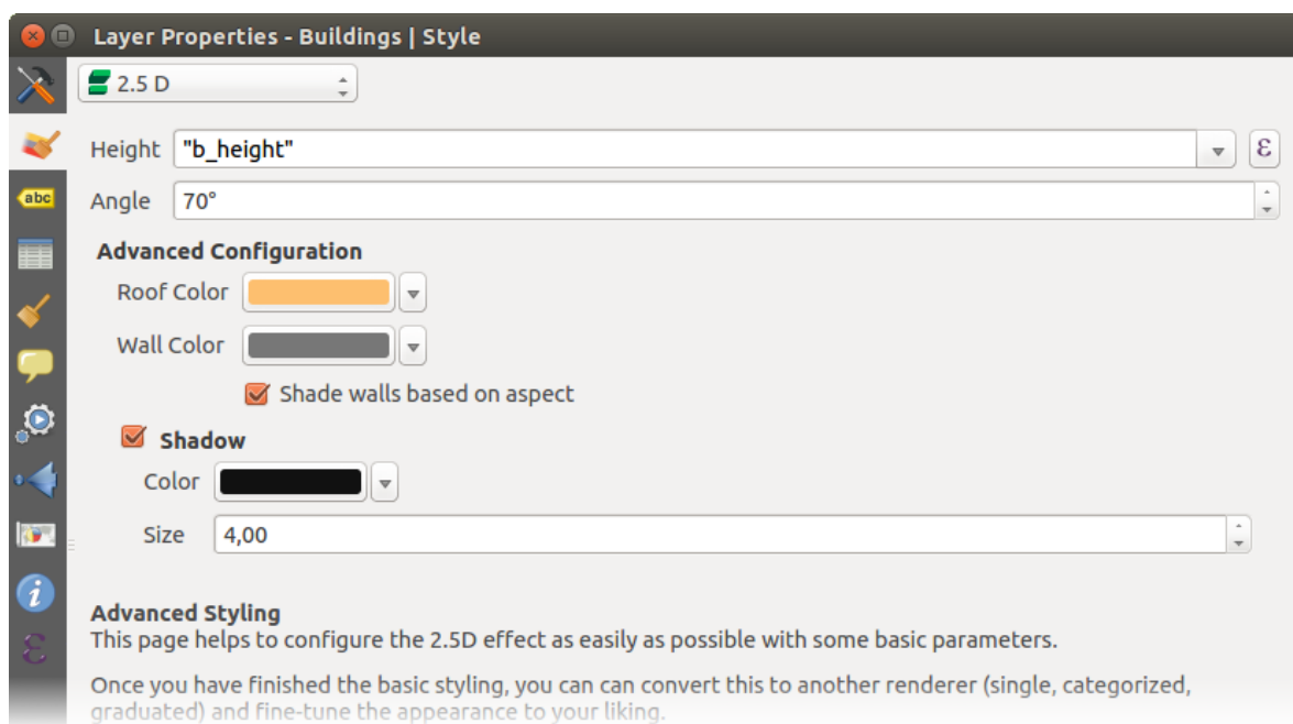
Gambar 12.23: 2.5 D dialog
