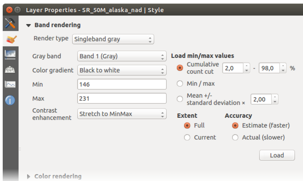
Gambar 13.4: Raster Renderer - Singleband gray
