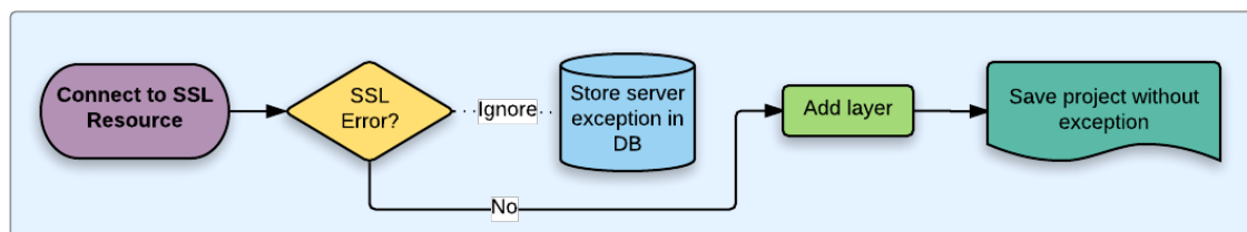
Gambar 16.33: SSL server exception
