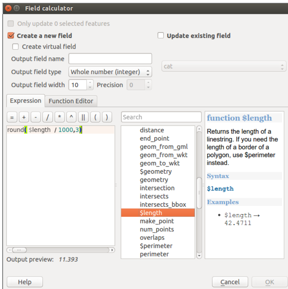
Gambar 12.61: Field Calculator
